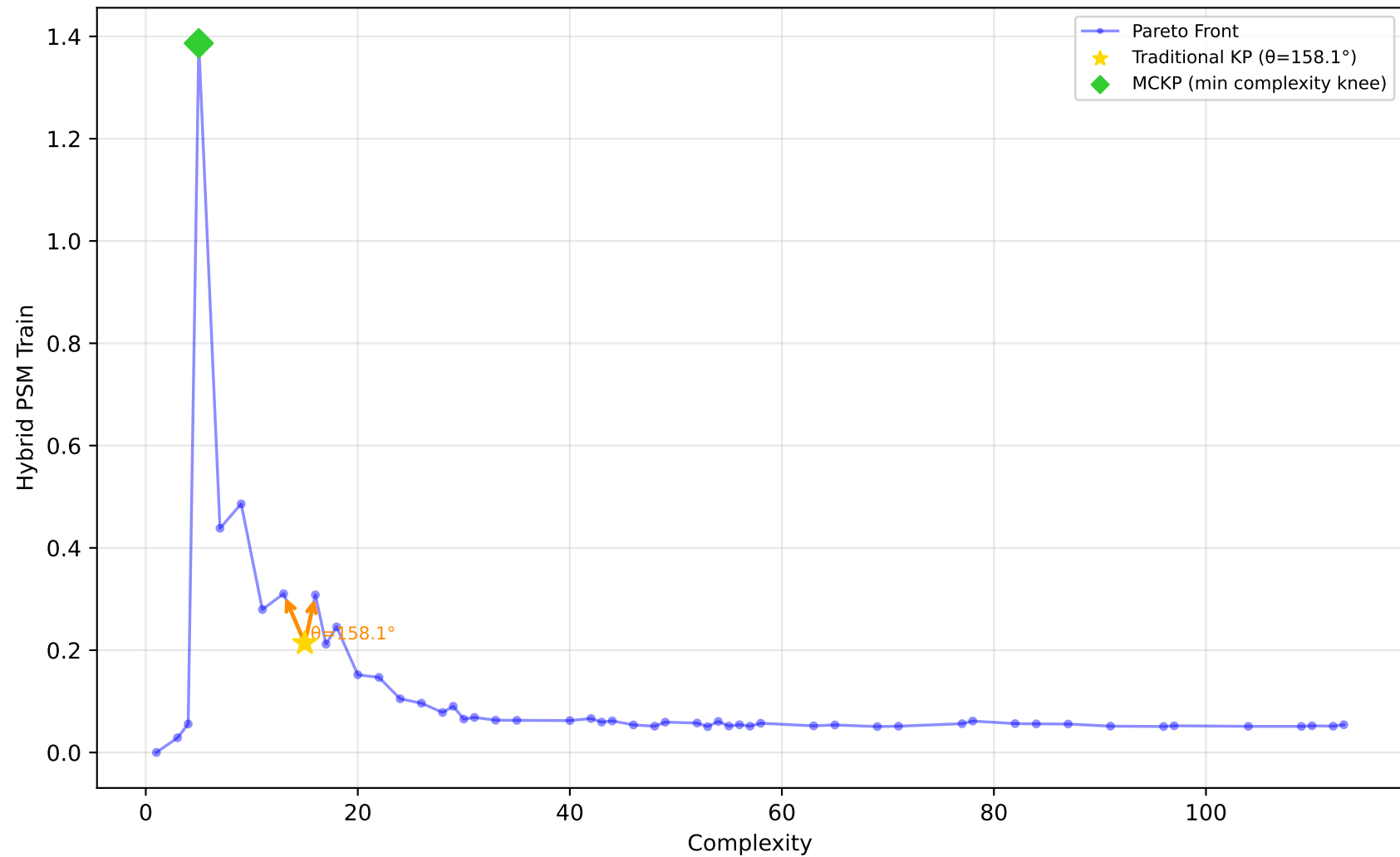
227_cpu_small - Run 19 - SVP - Hybrid PSM Train \lambda_1=0.00, \lambda_2=0.80, \lambda_3=0.30 | Difficulty: 1.00 | Method: hmr
