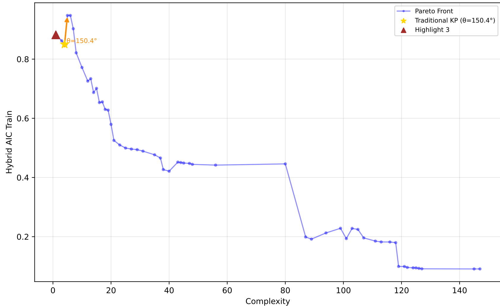
227_cpu_small - Run 1 - MVP - Hybrid AIC Train \lambda_1=0.00, \bar{\lambda}_2=0.90, \lambda_3=0.10 | Difficulty: 1.00 | Method: hmr
