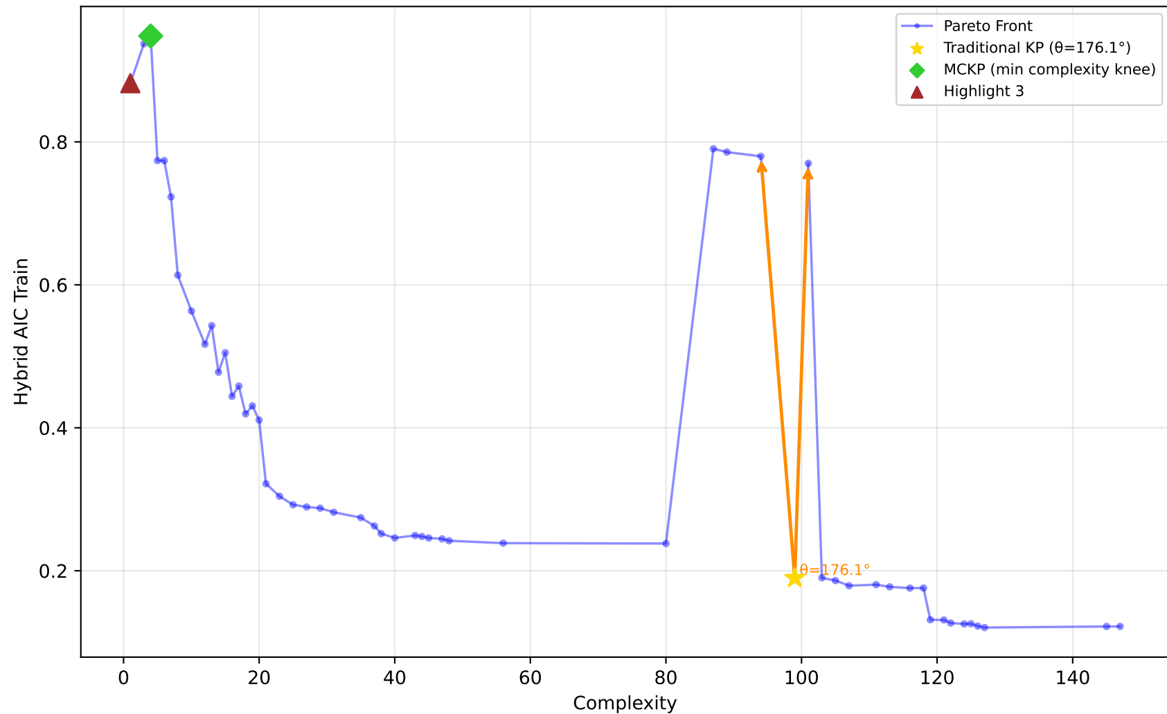
227_cpu_small - Run 1 - MVP - Hybrid AIC Train \lambda_1=0.80, \lambda_2=0.20, \lambda_3=0.00 | Difficulty: 1.00 | Method: hmr
