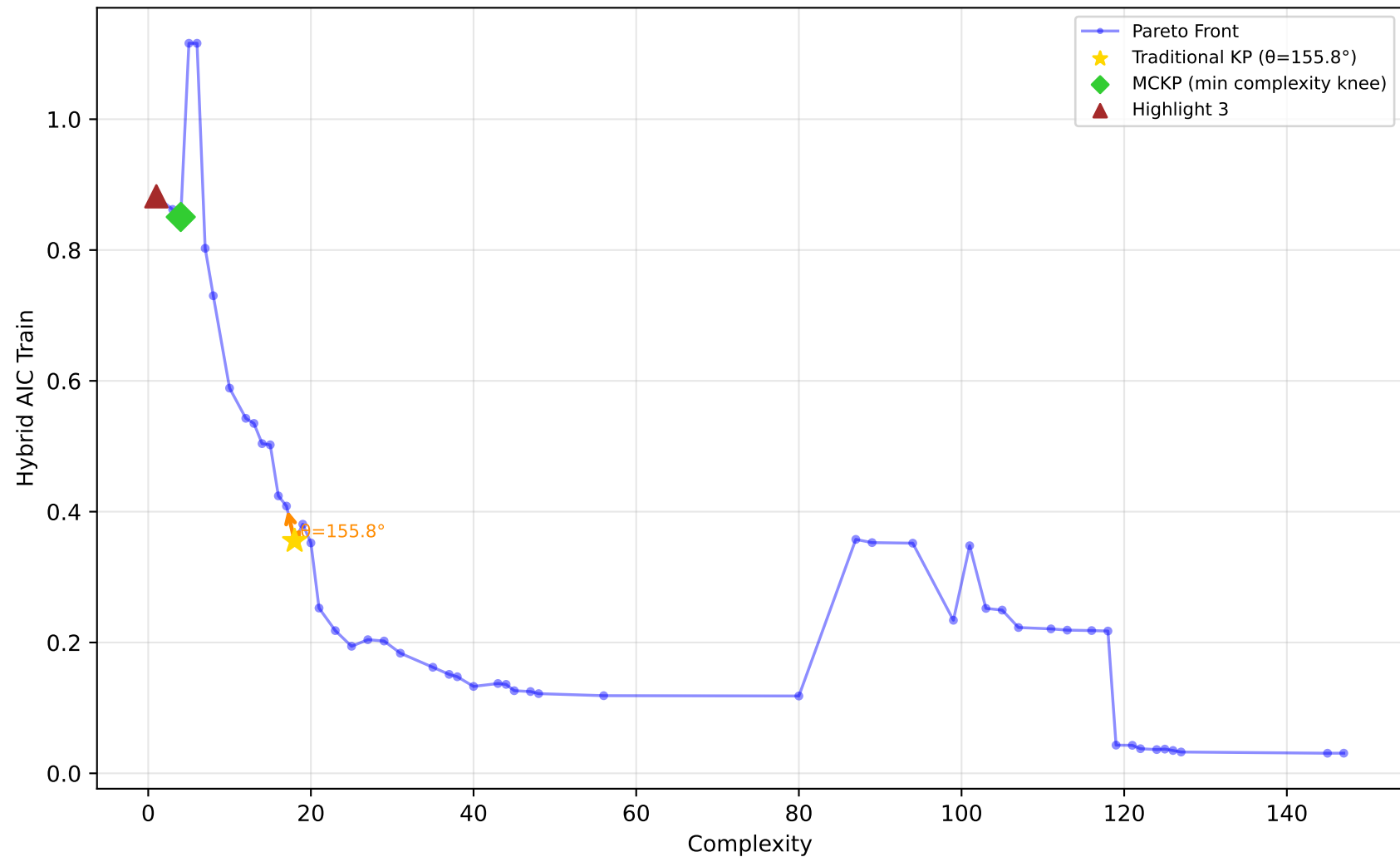
227_cpu_small - Run 1 - SVP - Hybrid AIC Train \lambda_1=0.00, \bar{\lambda}_2=0.80, \lambda_3=0.30 | Difficulty: 1.00 | Method: hmr
