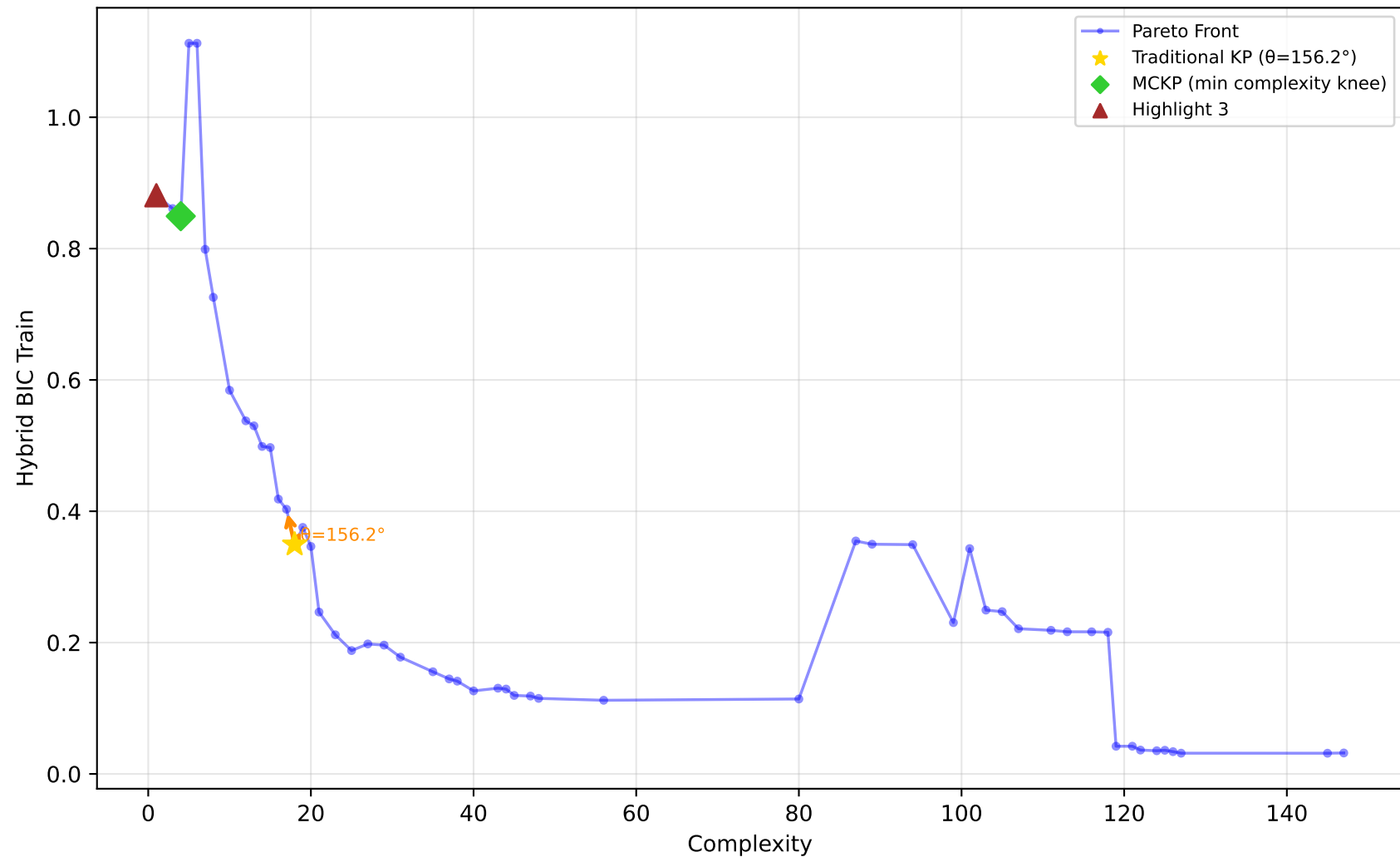
227_cpu_small - Run 1 - SVP - Hybrid BIC Train \lambda_1=0.00, \bar{\lambda}_2=0.80, \lambda_3=0.30 | Difficulty: 1.00 | Method: hmr
