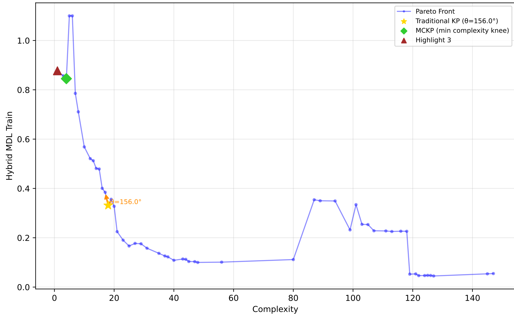
227_cpu_small - Run 1 - SVP - Hybrid MDL Train \lambda_1=0.00, \lambda_2=0.80, \lambda_3=0.30 | Difficulty: 1.00 | Method: hmr
