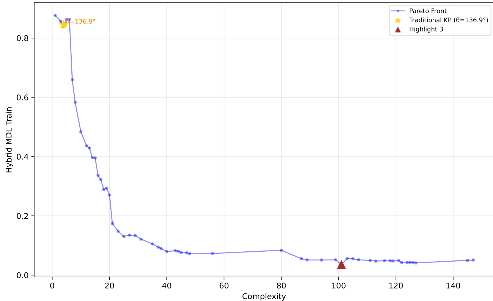
227_cpu_small - Run 1 - SVP - Hybrid MDL Train \lambda_1=0.00, \lambda_2=1.00, \lambda_3=0.00 | Difficulty: 1.00 | Method: hmr
