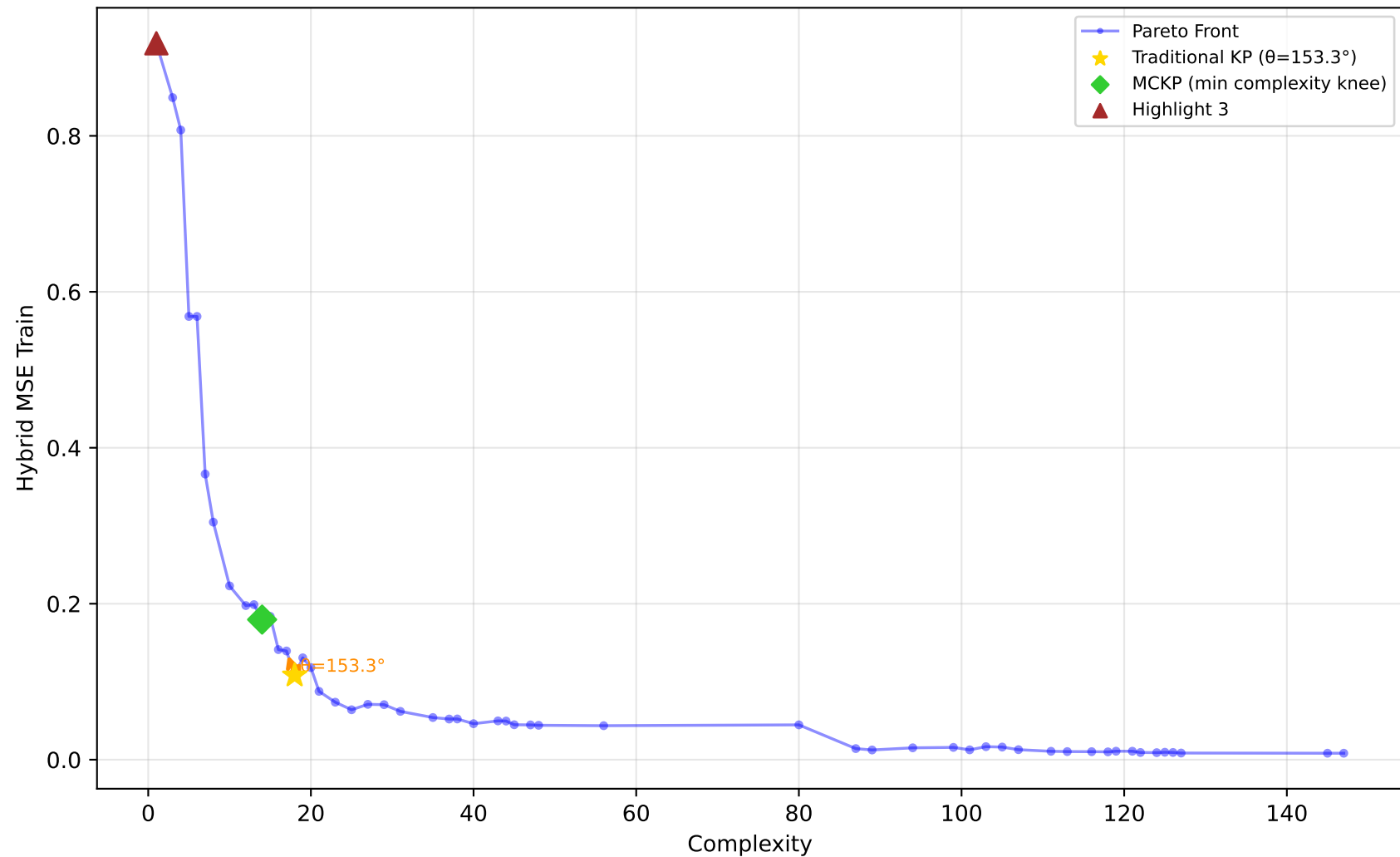
227_cpu_small - Run 1 - SVP - Hybrid MSE Train \lambda_1=0.00, \bar{\lambda}_2=1.00, \lambda_3=0.00 | Difficulty: 1.00 | Method: hmr
