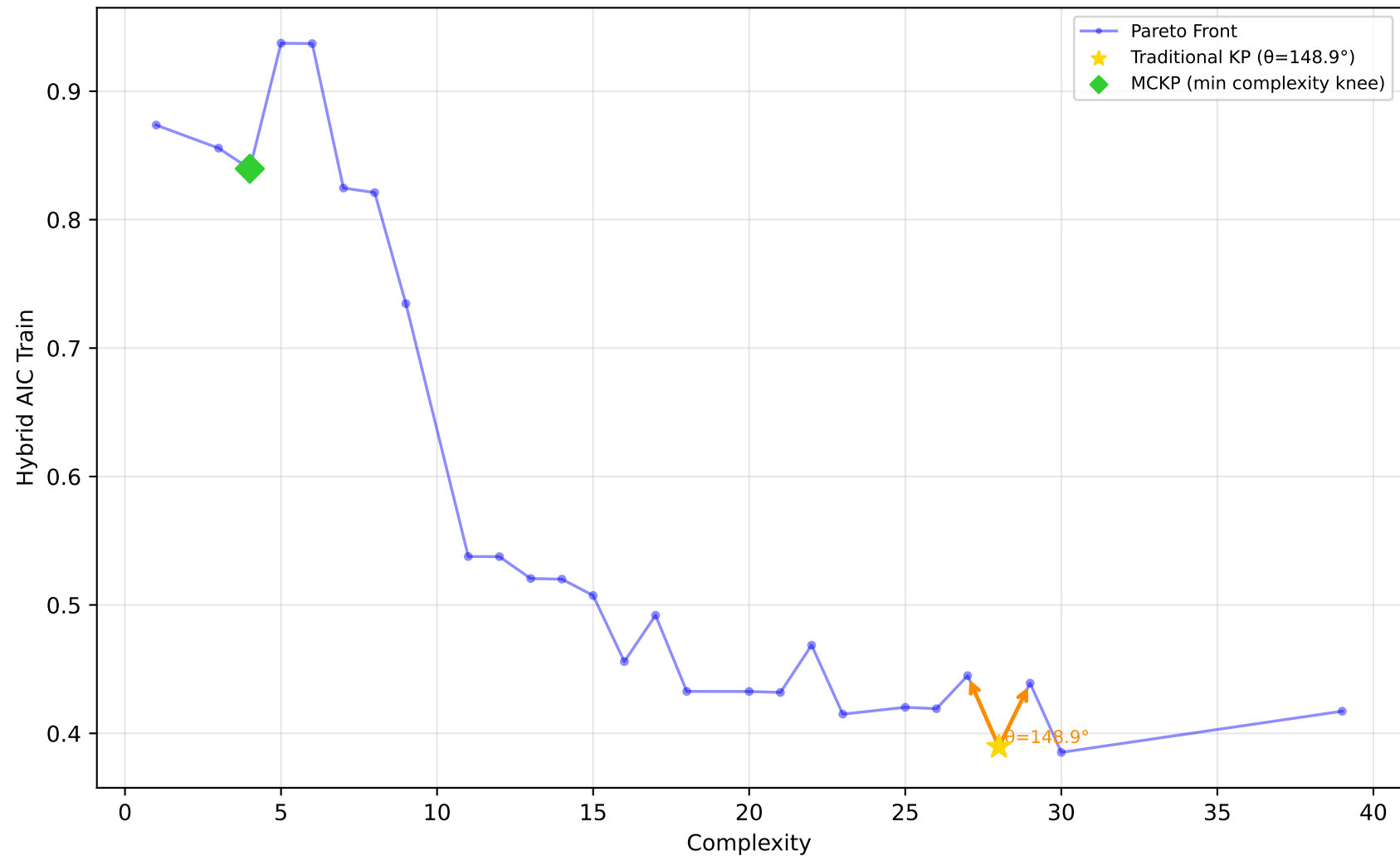
227_cpu_small - Run 20 - MVP - Hybrid AIC Train \lambda_1=0.00, \bar{\lambda}_2=0.90, \lambda_3=0.10 | Difficulty: 1.00 | Method: hmr
