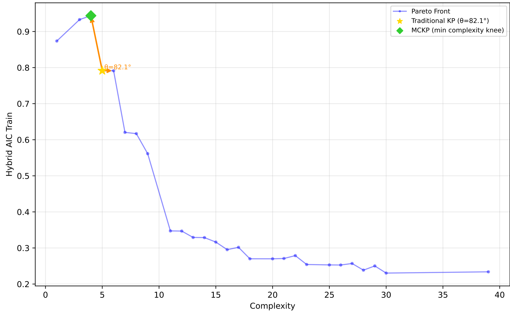
227_cpu_small - Run 20 - MVP - Hybrid AIC Train \lambda_1=0.80, \bar{\lambda}_2=0.20, \lambda_3=0.00 | Difficulty: 1.00 | Method: hmr
