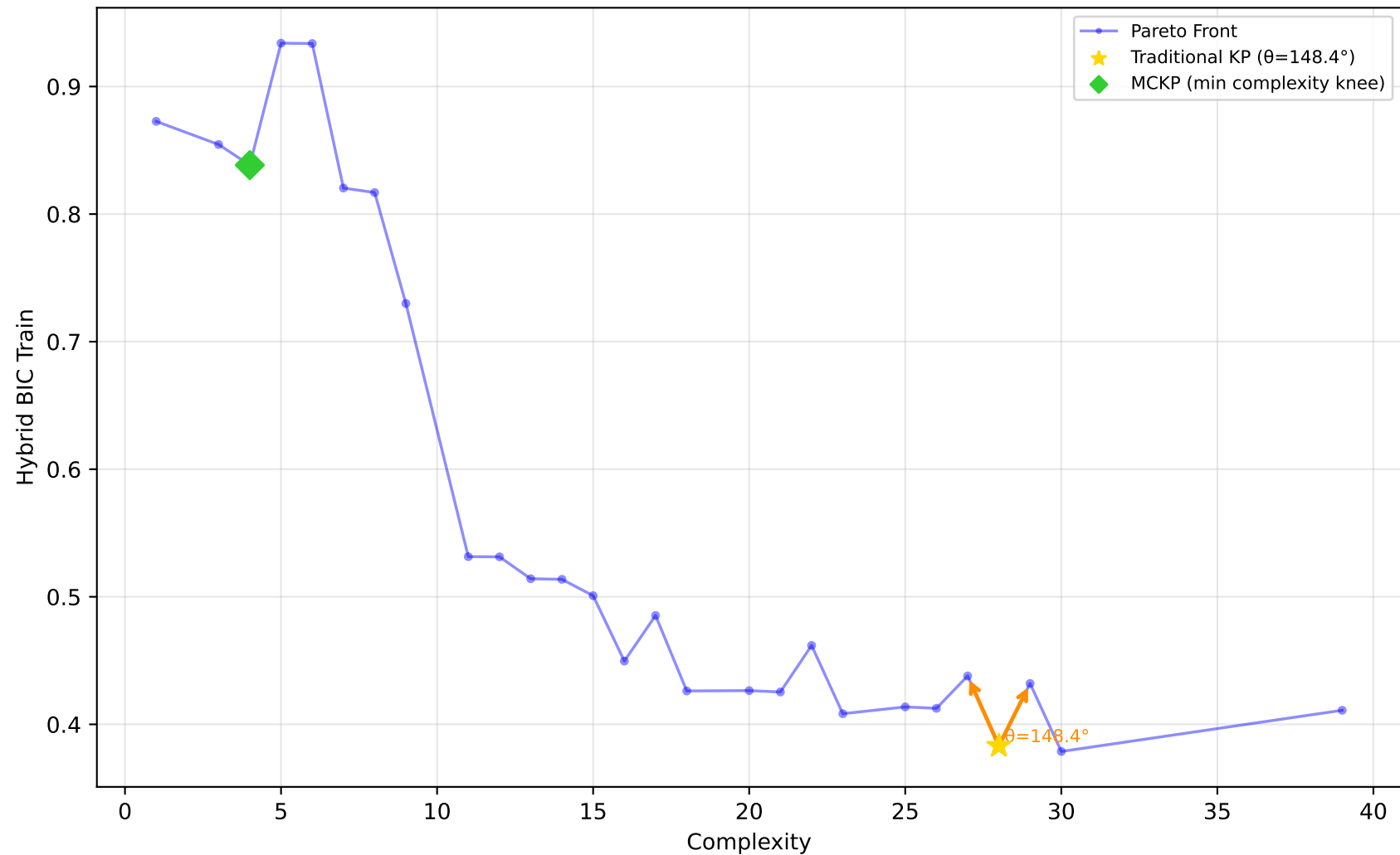
227_cpu_small - Run 20 - MVP - Hybrid BIC Train \lambda_1=0.00, \lambda_2=0.90, \lambda_3=0.10 | Difficulty: 1.00 | Method: hmr
