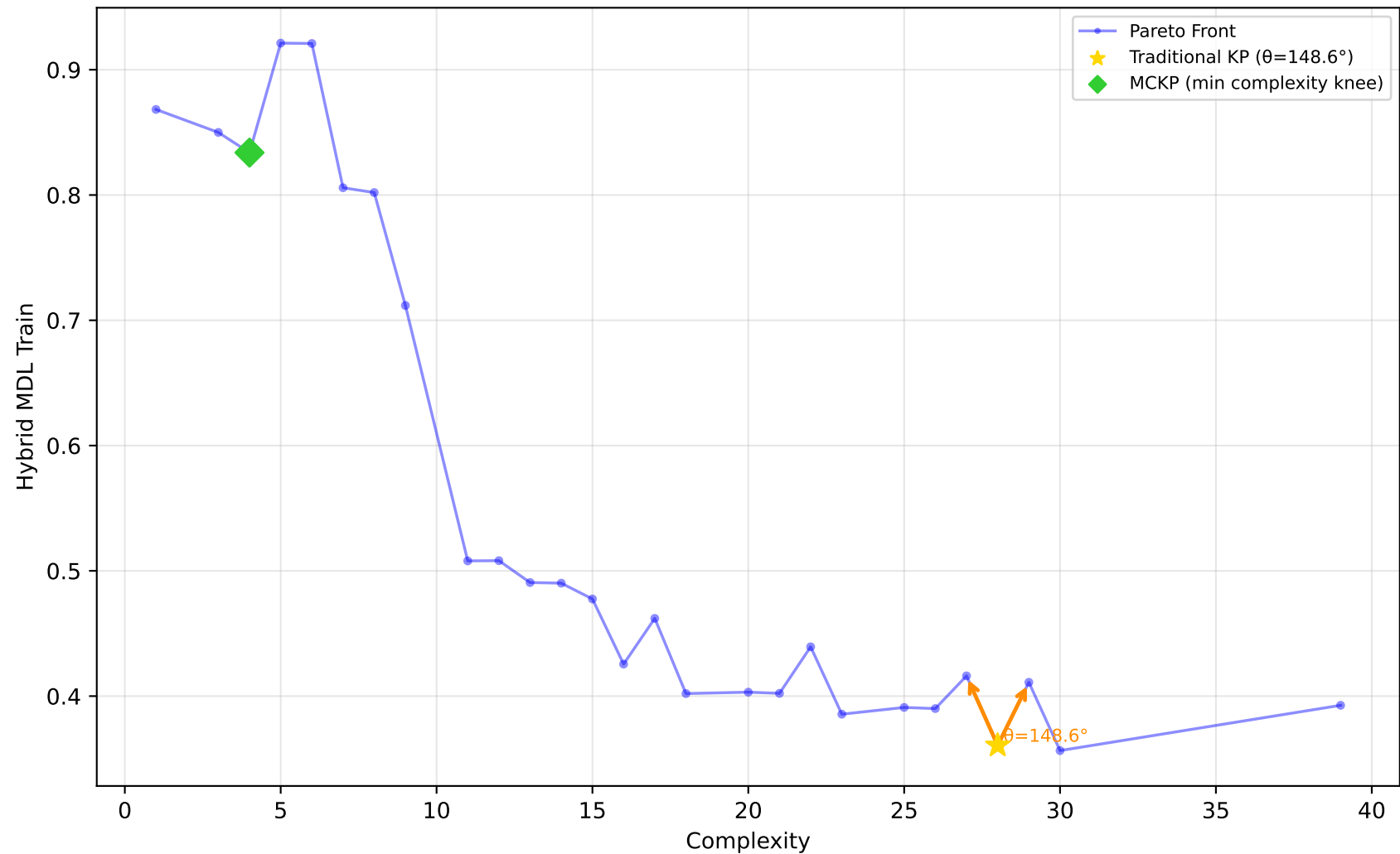
227_cpu_small - Run 20 - MVP - Hybrid MDL Train \lambda_1=0.00, \lambda_2=0.90, \lambda_3=0.10 | Difficulty: 1.00 | Method: hmr
