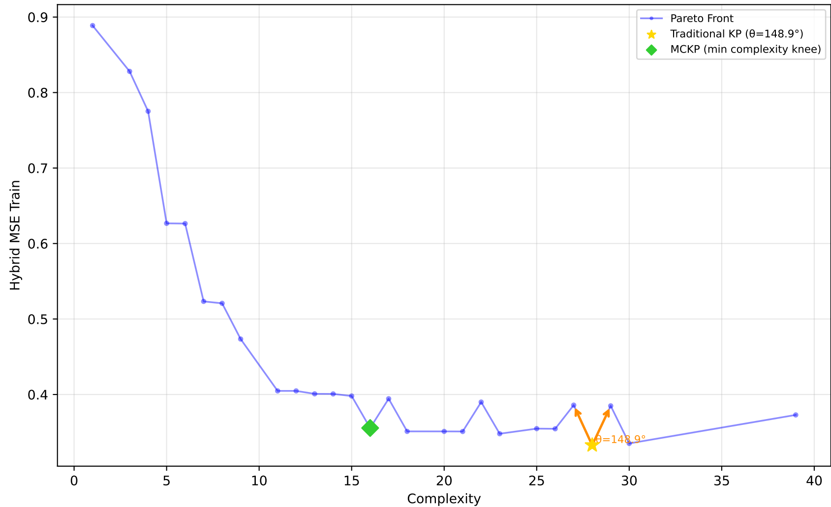
227_cpu_small - Run 20 - MVP - Hybrid MSE Train \lambda_1=0.00, \lambda_2=0.90, \lambda_3=0.10 | Difficulty: 1.00 | Method: hmr
