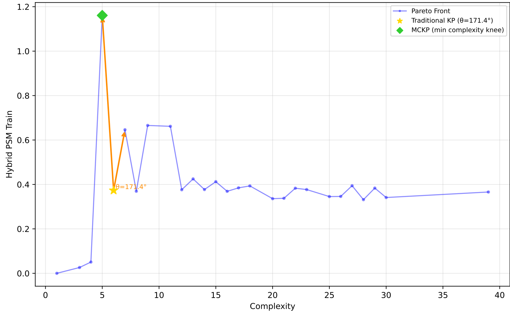
227_cpu_small - Run 20 - MVP - Hybrid PSM Train \lambda_1=0.00, \lambda_2=0.90, \lambda_3=0.10 | Difficulty: 1.00 | Method: hmr
