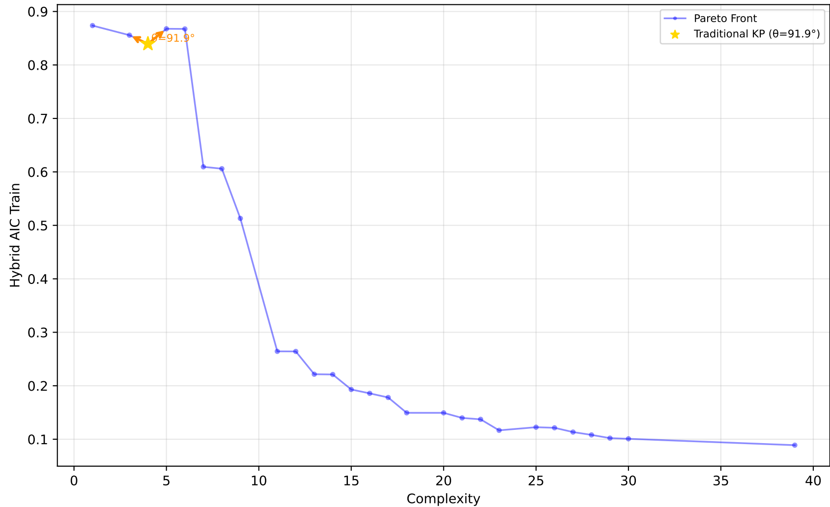
227_cpu_small - Run 20 - SVP - Hybrid AIC Train \lambda_1=0.00, \lambda_2=1.00, \lambda_3=0.00 | Difficulty: 1.00 | Method: hmr
