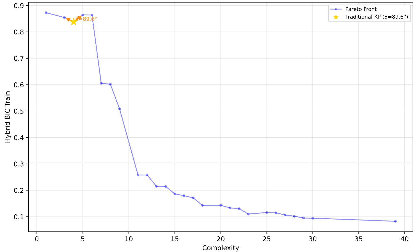
227_cpu_small - Run 20 - SVP - Hybrid BIC Train \lambda_1=0.00, \lambda_2=1.00, \lambda_3=0.00 | Difficulty: 1.00 | Method: hmr
