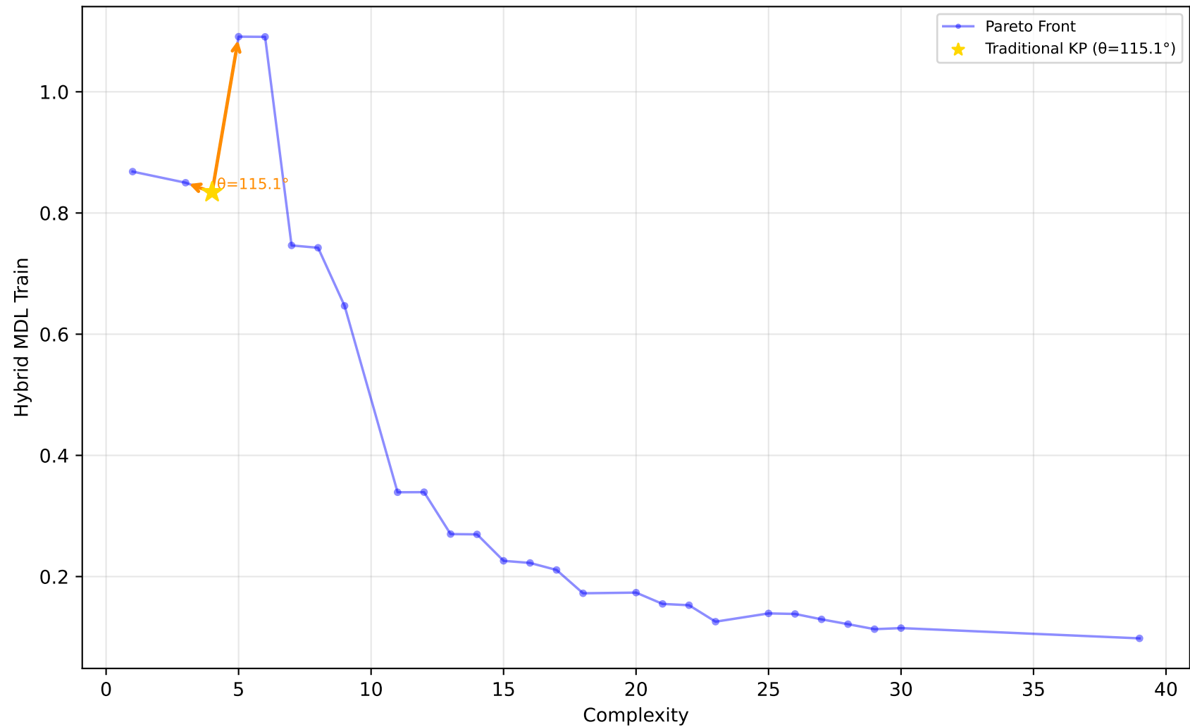
227_cpu_small - Run 20 - SVP - Hybrid MDL Train \lambda_1=0.00, \lambda_2=0.80, \lambda_3=0.30 | Difficulty: 1.00 | Method: hmr
