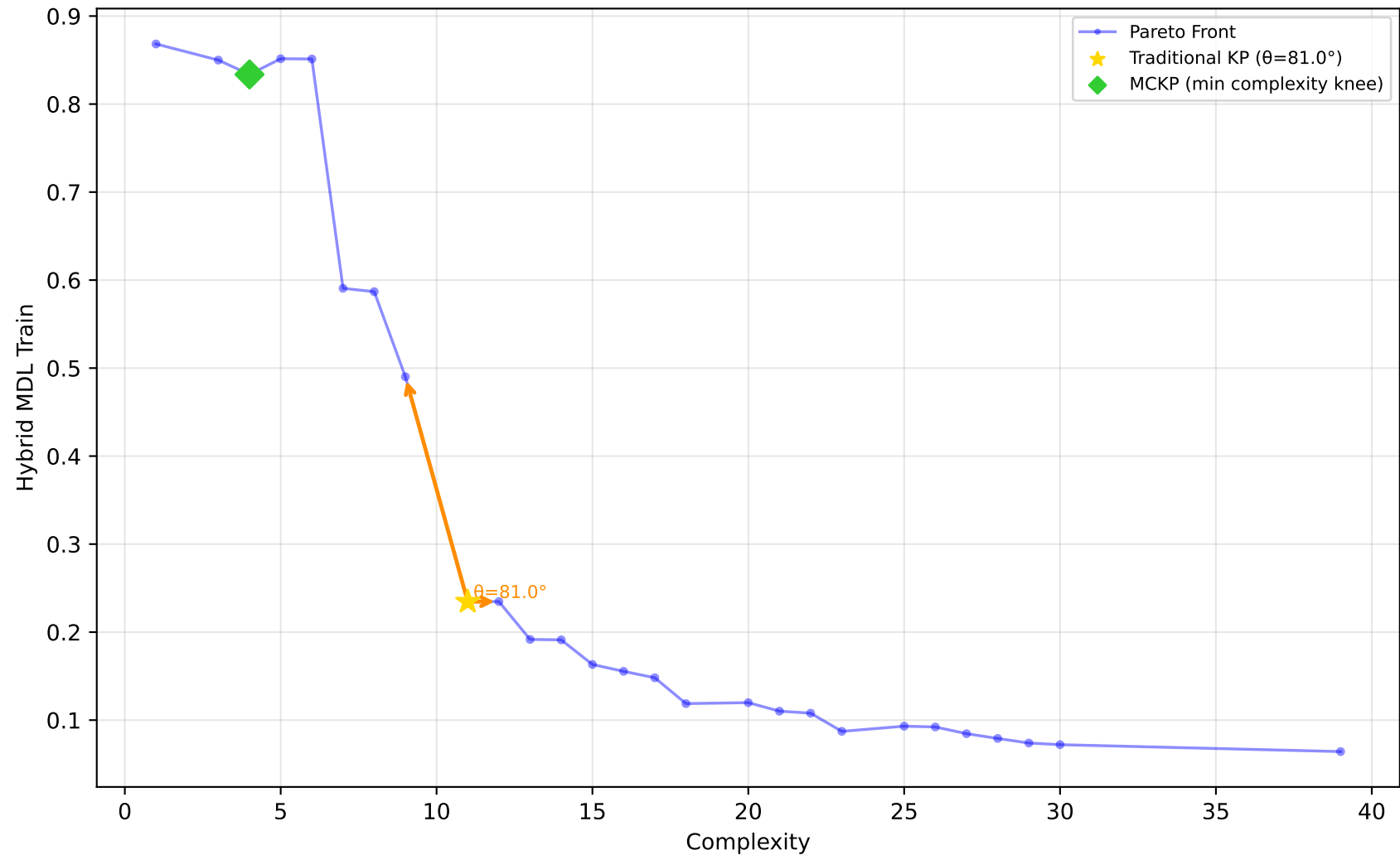
227_cpu_small - Run 20 - SVP - Hybrid MDL Train \lambda_1=0.00, \lambda_2=1.00, \lambda_3=0.00 | Difficulty: 1.00 | Method: hmr
