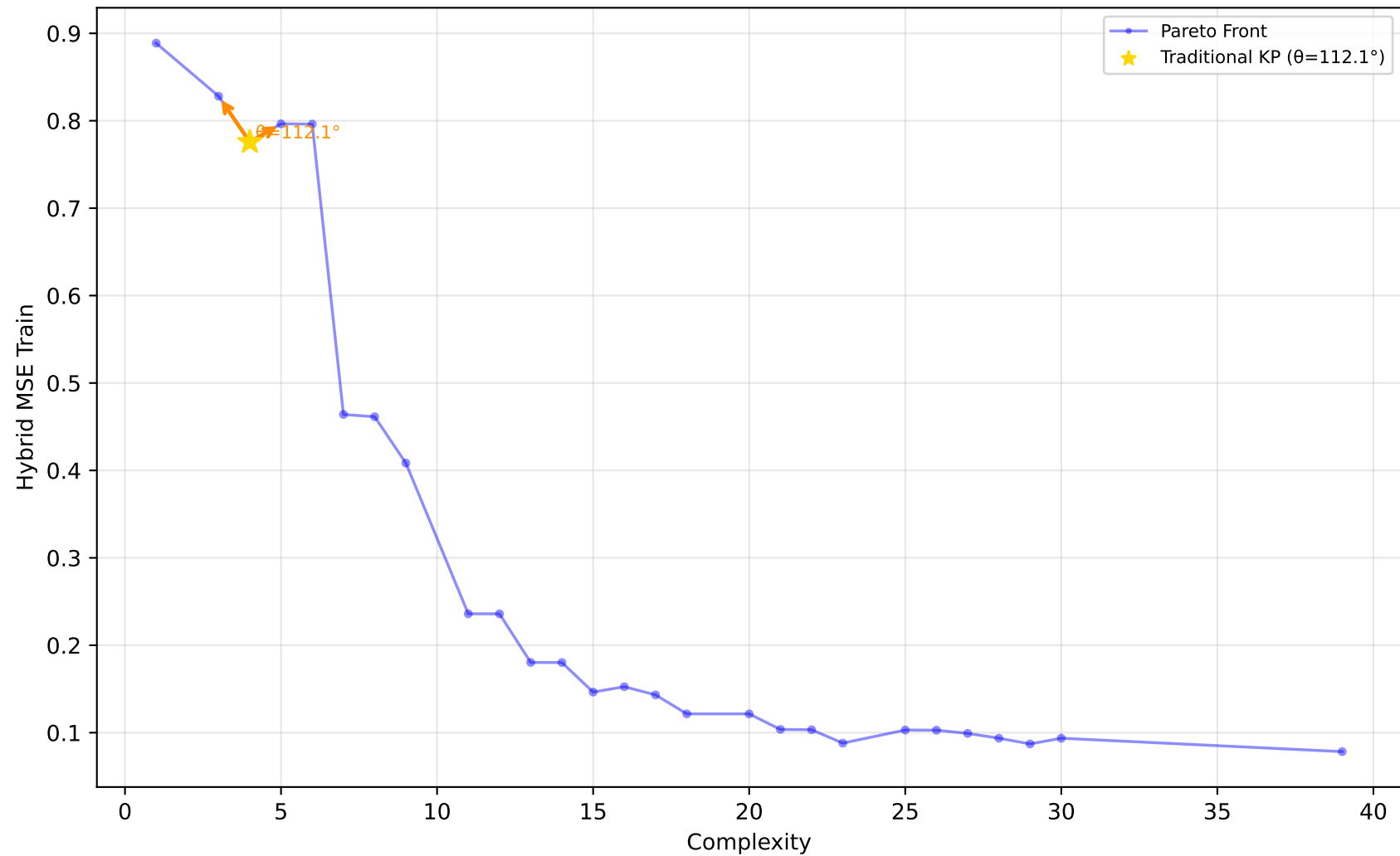
227_cpu_small - Run 20 - SVP - Hybrid MSE Train \lambda_1=0.00, \lambda_2=0.80, \lambda_3=0.30 | Difficulty: 1.00 | Method: hmr
