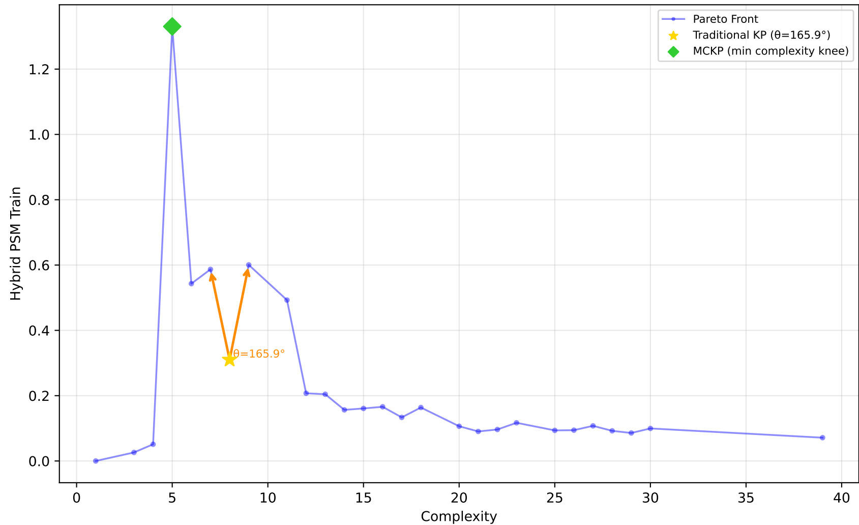
227_cpu_small - Run 20 - SVP - Hybrid PSM Train \lambda_1=0.00, \lambda_2=0.80, \lambda_3=0.30 | Difficulty: 1.00 | Method: hmr
