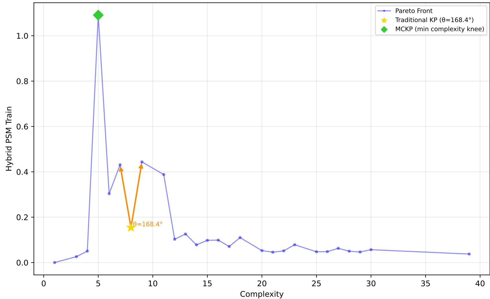
227_cpu_small - Run 20 - SVP - Hybrid PSM Train \lambda_1=0.00, \lambda_2=1.00, \lambda_3=0.00 | Difficulty: 1.00 | Method: hmr
