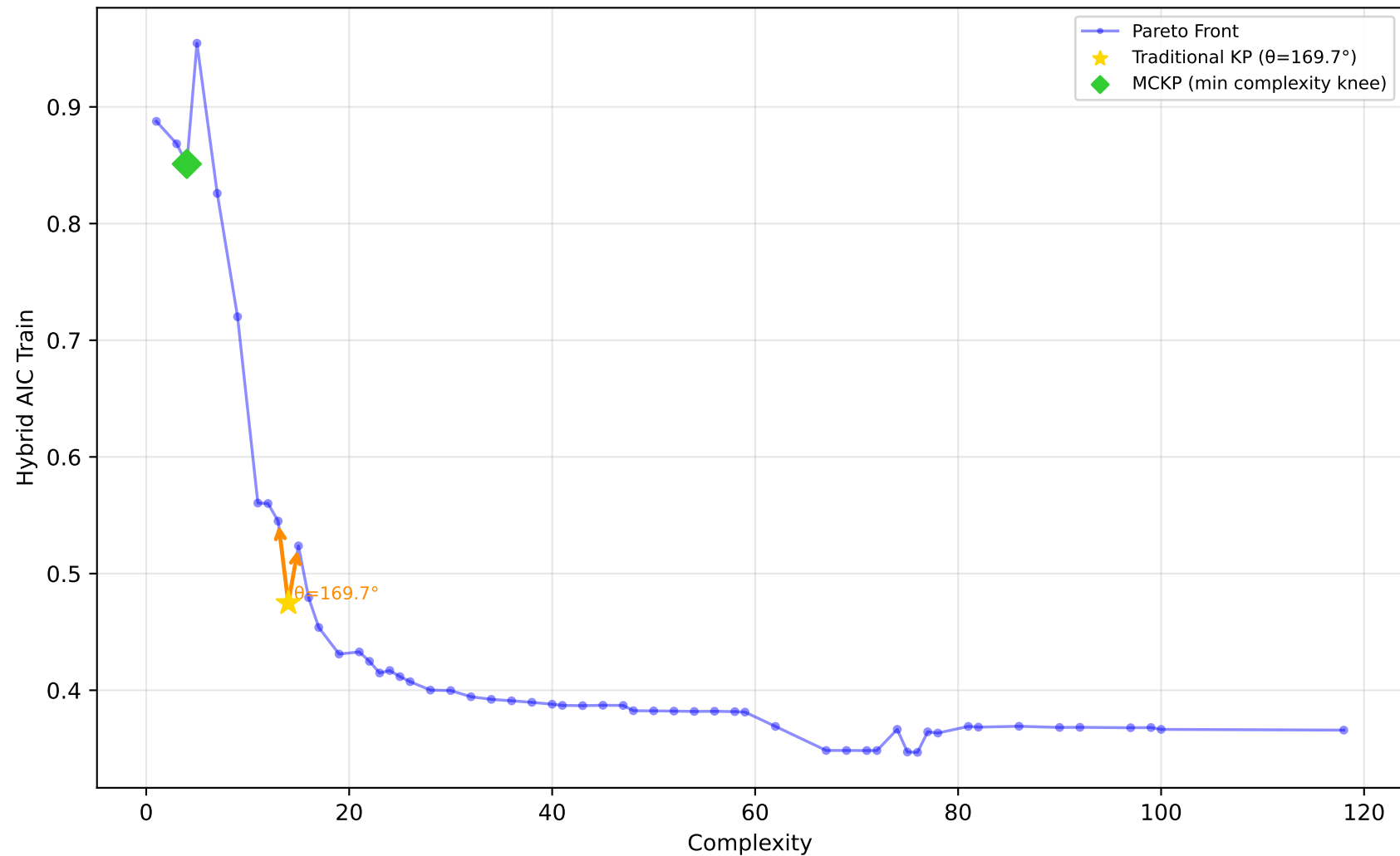
227_cpu_small - Run 21 - MVP - Hybrid AIC Train \lambda_1=0.00, \lambda_2=0.90, \lambda_3=0.10 | Difficulty: 1.00 | Method: hmr
