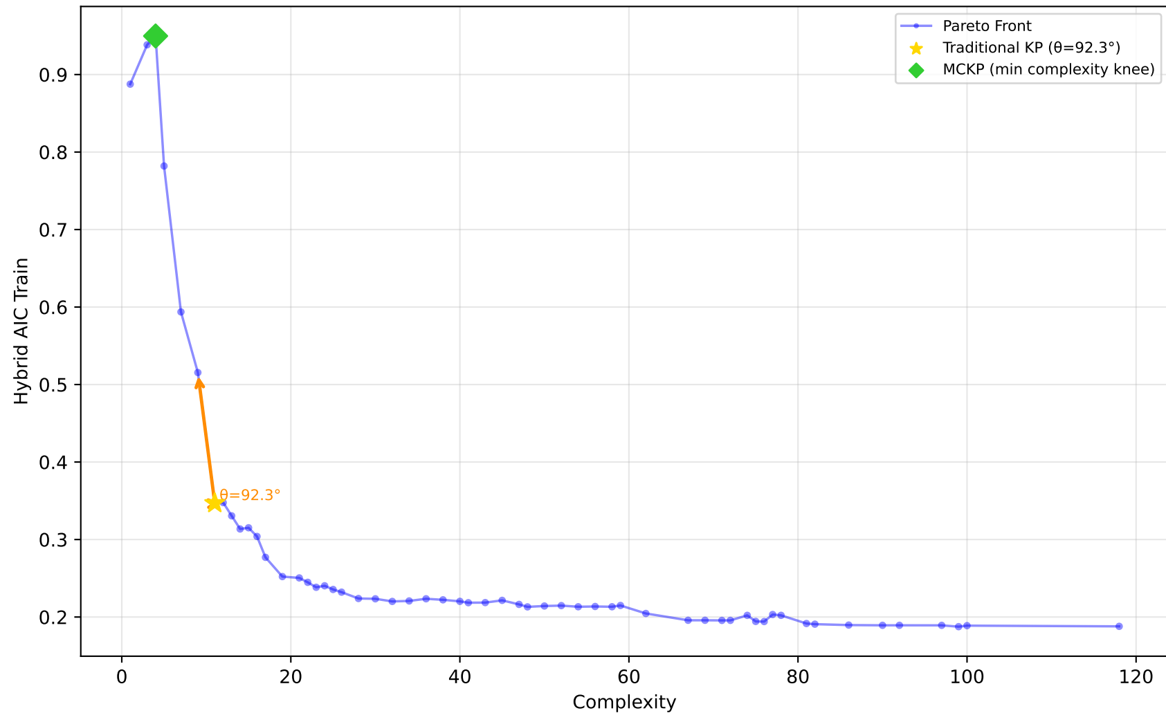
227_cpu_small - Run 21 - MVP - Hybrid AIC Train \lambda_1=0.80, \lambda_2=0.20, \lambda_3=0.00 | Difficulty: 1.00 | Method: hmr
