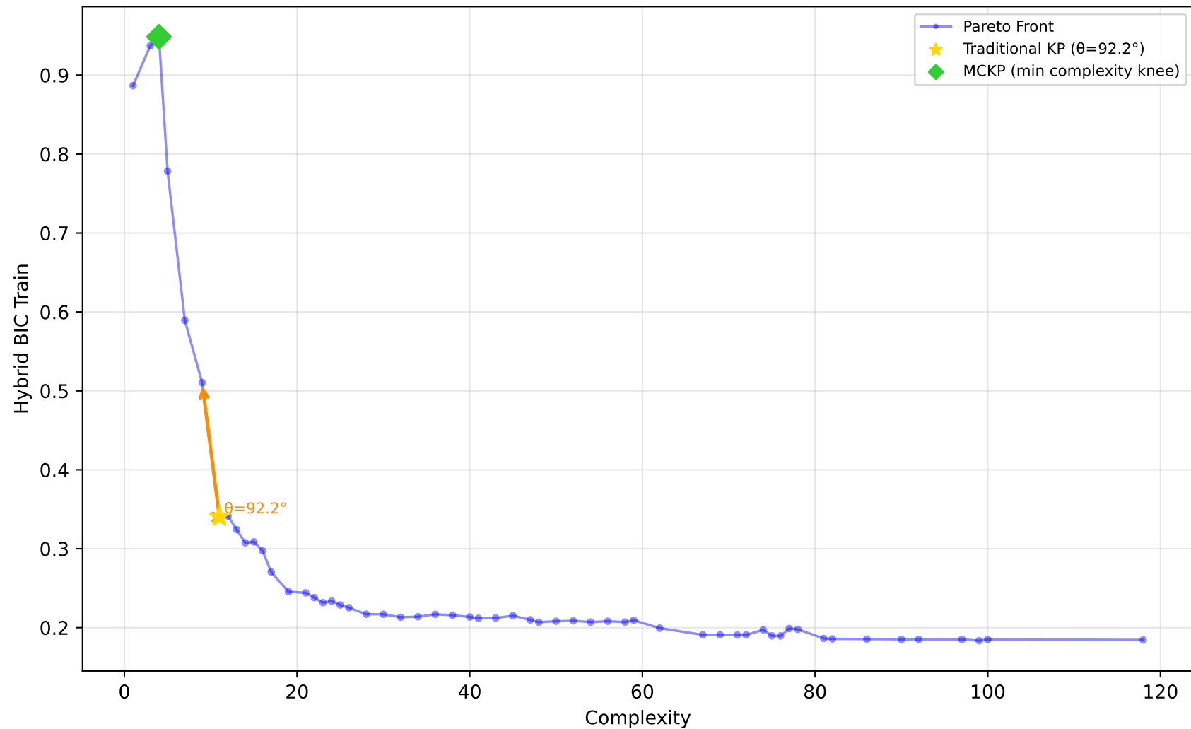
227_cpu_small - Run 21 - MVP - Hybrid BIC Train \lambda_1=0.80, \lambda_2=0.20, \lambda_3=0.00 | Difficulty: 1.00 | Method: hmr
