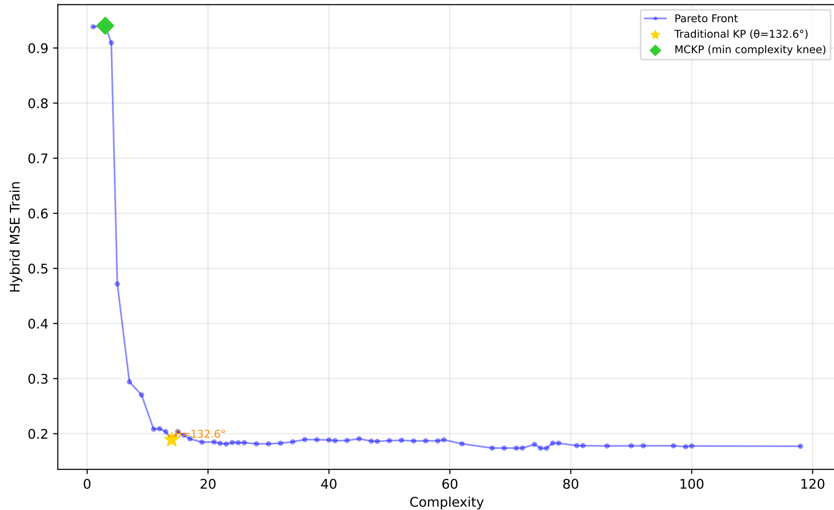
227_cpu_small - Run 21 - MVP - Hybrid MSE Train \lambda_1=0.80, \lambda_2=0.20, \lambda_3=0.00 | Difficulty: 1.00 | Method: hmr
