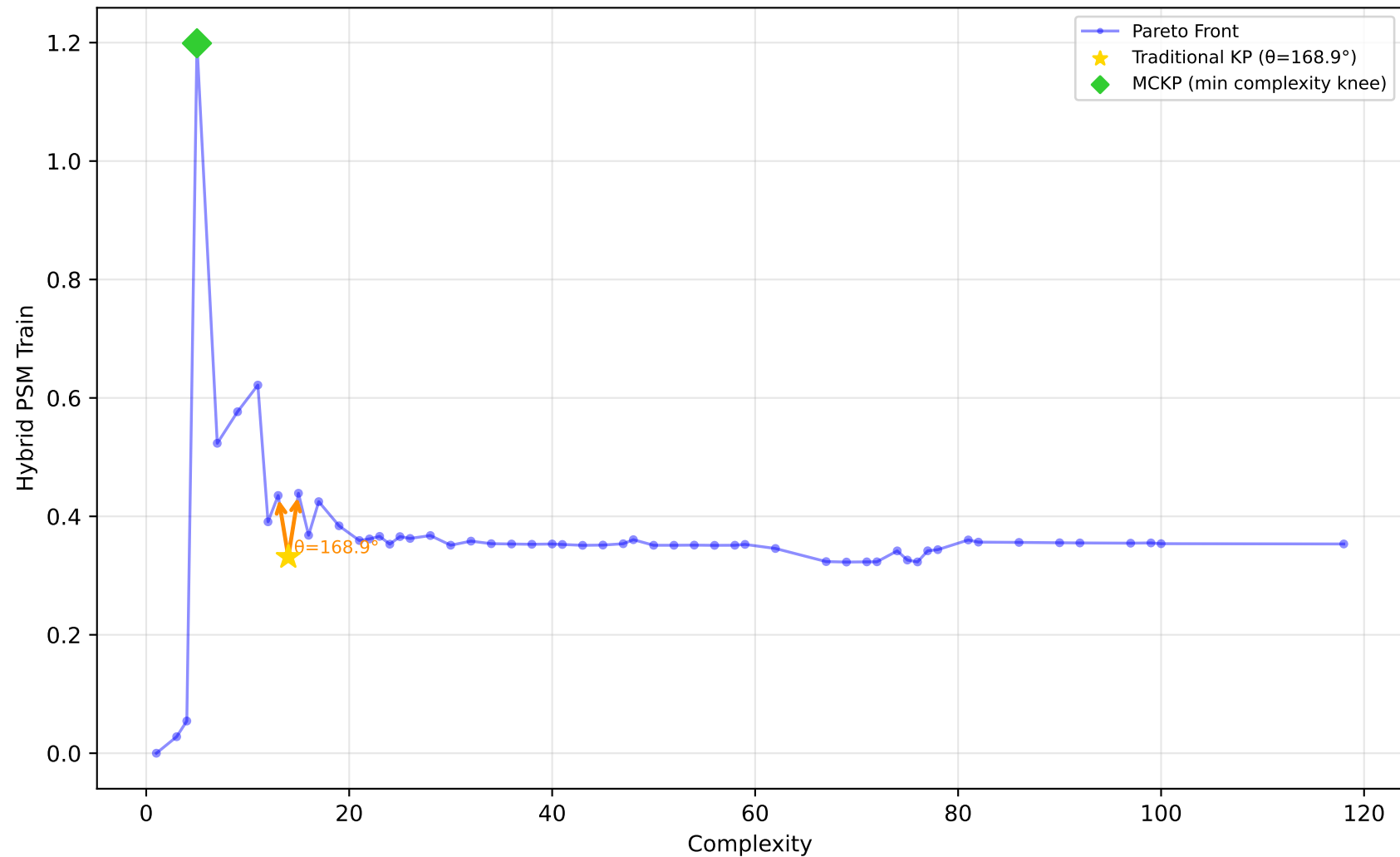
227_cpu_small - Run 21 - MVP - Hybrid PSM Train \lambda_1=0.00, \lambda_2=0.90, \lambda_3=0.10 | Difficulty: 1.00 | Method: hmr
