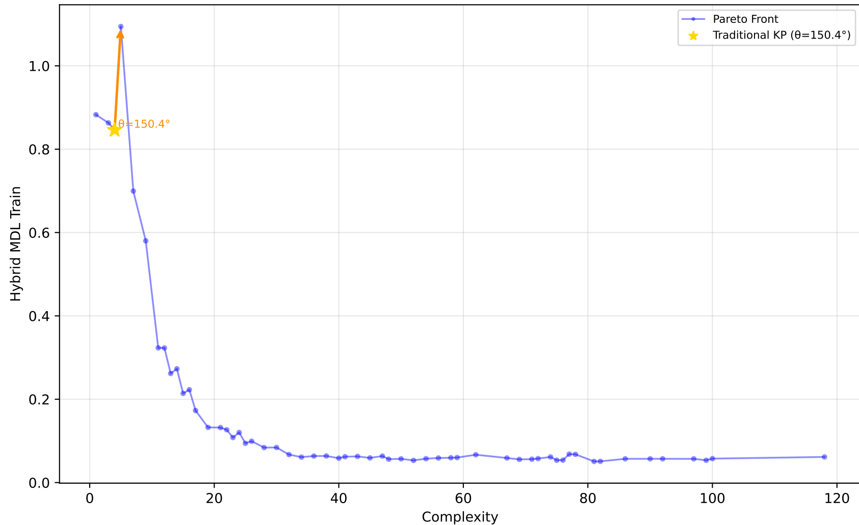
227_cpu_small - Run 21 - SVP - Hybrid MDL Train \lambda_1=0.00, \lambda_2=0.80, \lambda_3=0.30 | Difficulty: 1.00 | Method: hmr
