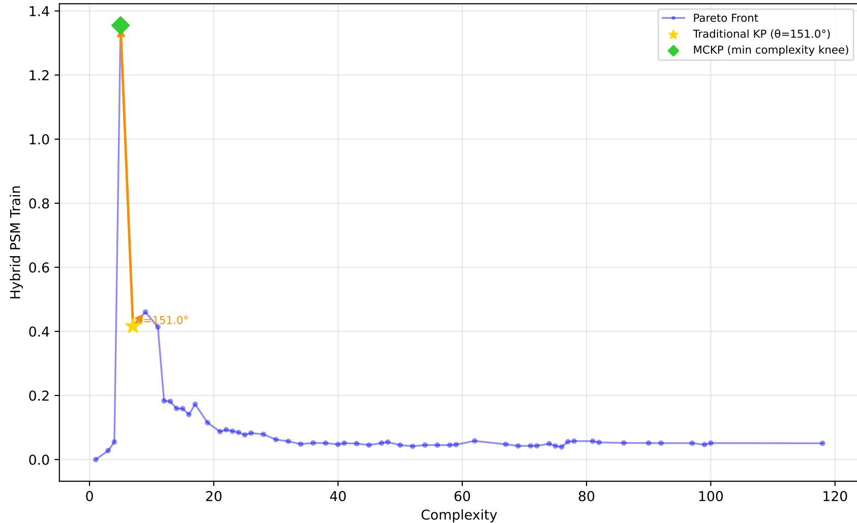
227_cpu_small - Run 21 - SVP - Hybrid PSM Train \lambda_1=0.00, \lambda_2=0.80, \lambda_3=0.30 | Difficulty: 1.00 | Method: hmr
