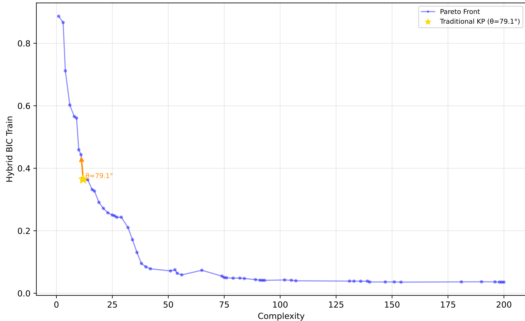
227_cpu_small - Run 22 - MVP - Hybrid BIC Train \lambda_1=0.00, \bar{\lambda}_2=0.90, \lambda_3=0.10 | Difficulty: 1.00 | Method: hmr
