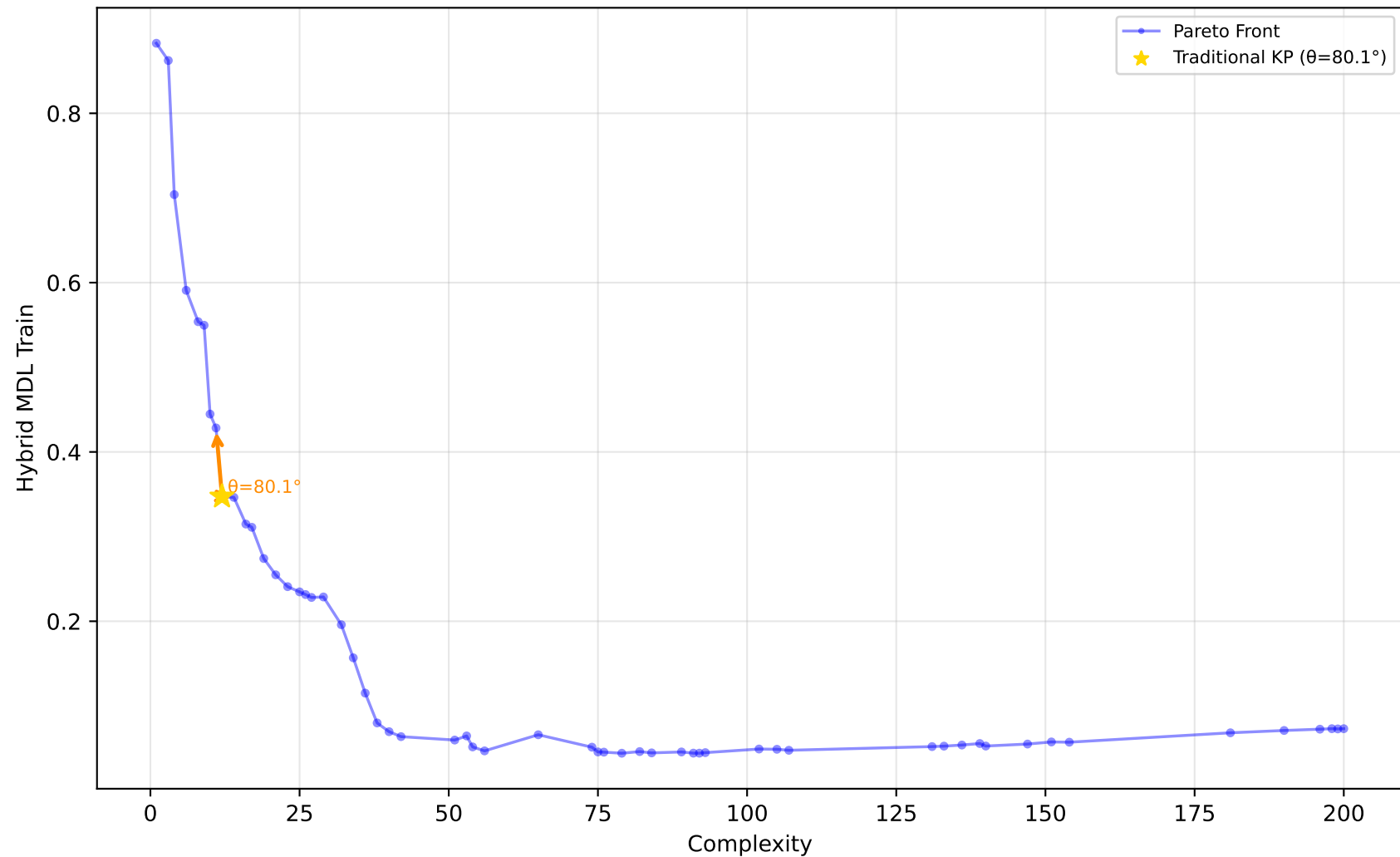
227_cpu_small - Run 22 - MVP - Hybrid MDL Train \lambda_1=0.00, \lambda_2=0.90, \lambda_3=0.10 | Difficulty: 1.00 | Method: hmr
