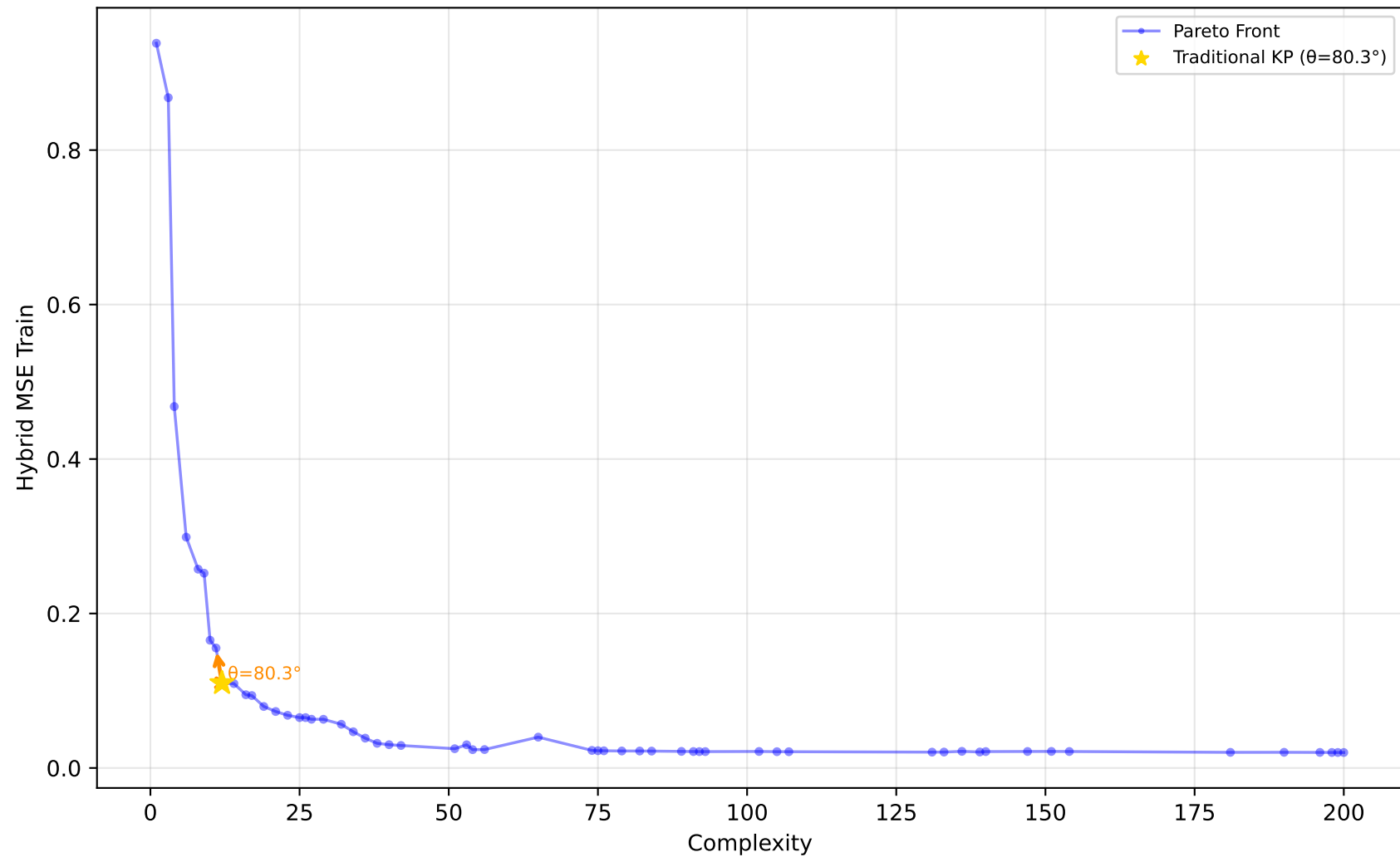
227_cpu_small - Run 22 - MVP - Hybrid MSE Train \lambda_1=0.00, \lambda_2=0.90, \lambda_3=0.10 | Difficulty: 1.00 | Method: hmr
