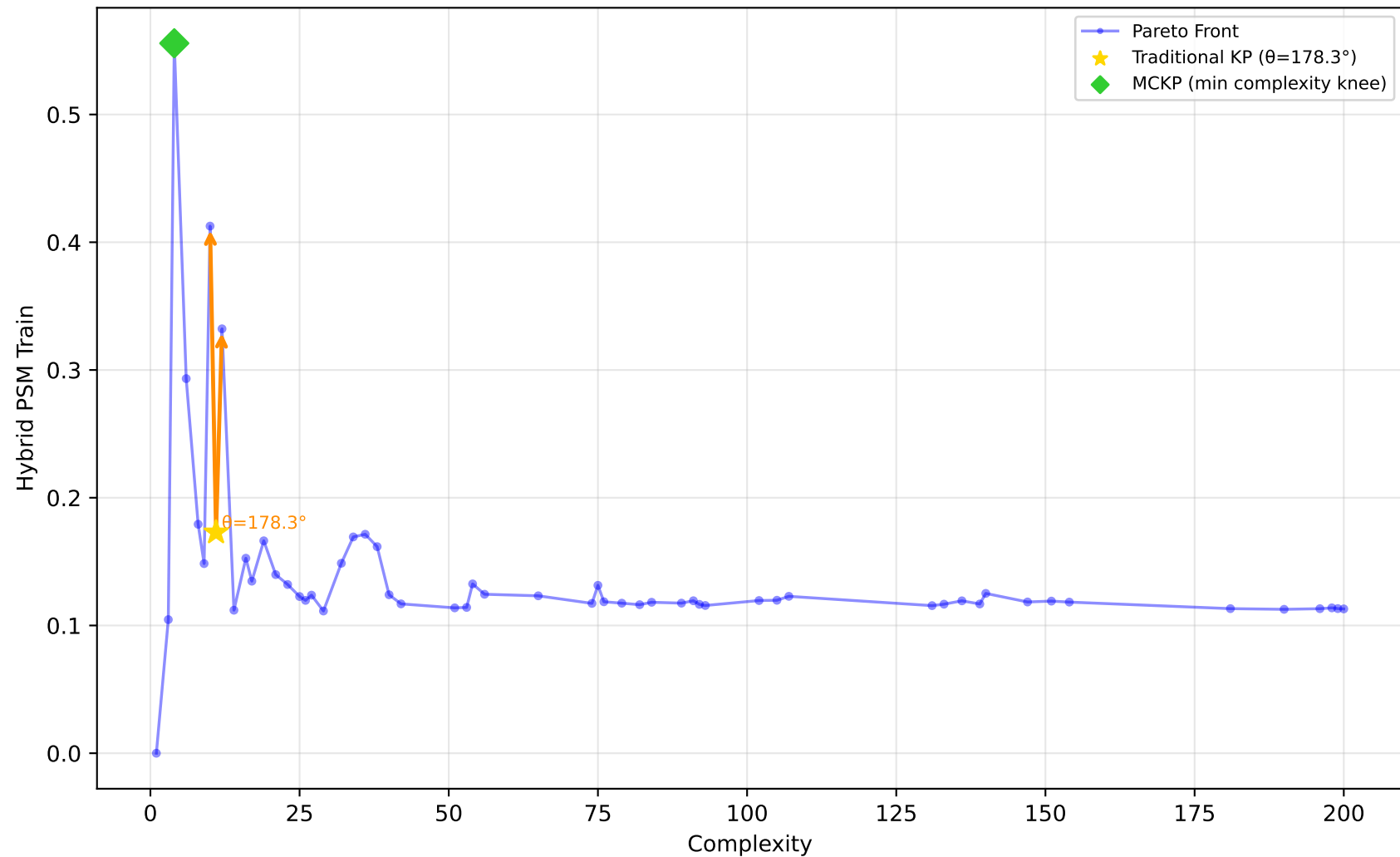
227_cpu_small - Run 22 - MVP - Hybrid PSM Train \lambda_1=0.80, \lambda_2=0.20, \lambda_3=0.00 | Difficulty: 1.00 | Method: hmr
