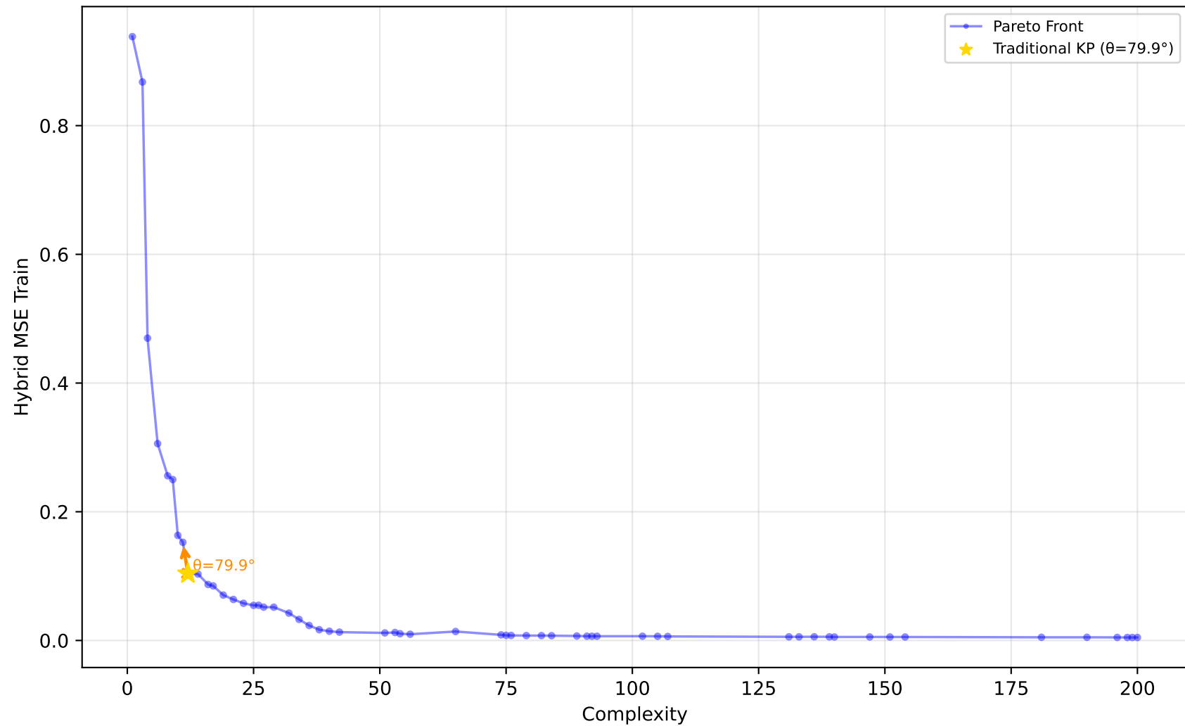
227_cpu_small - Run 22 - SVP - Hybrid MSE Train \lambda_1=0.00, \lambda_2=0.80, \lambda_3=0.30 | Difficulty: 1.00 | Method: hmr
