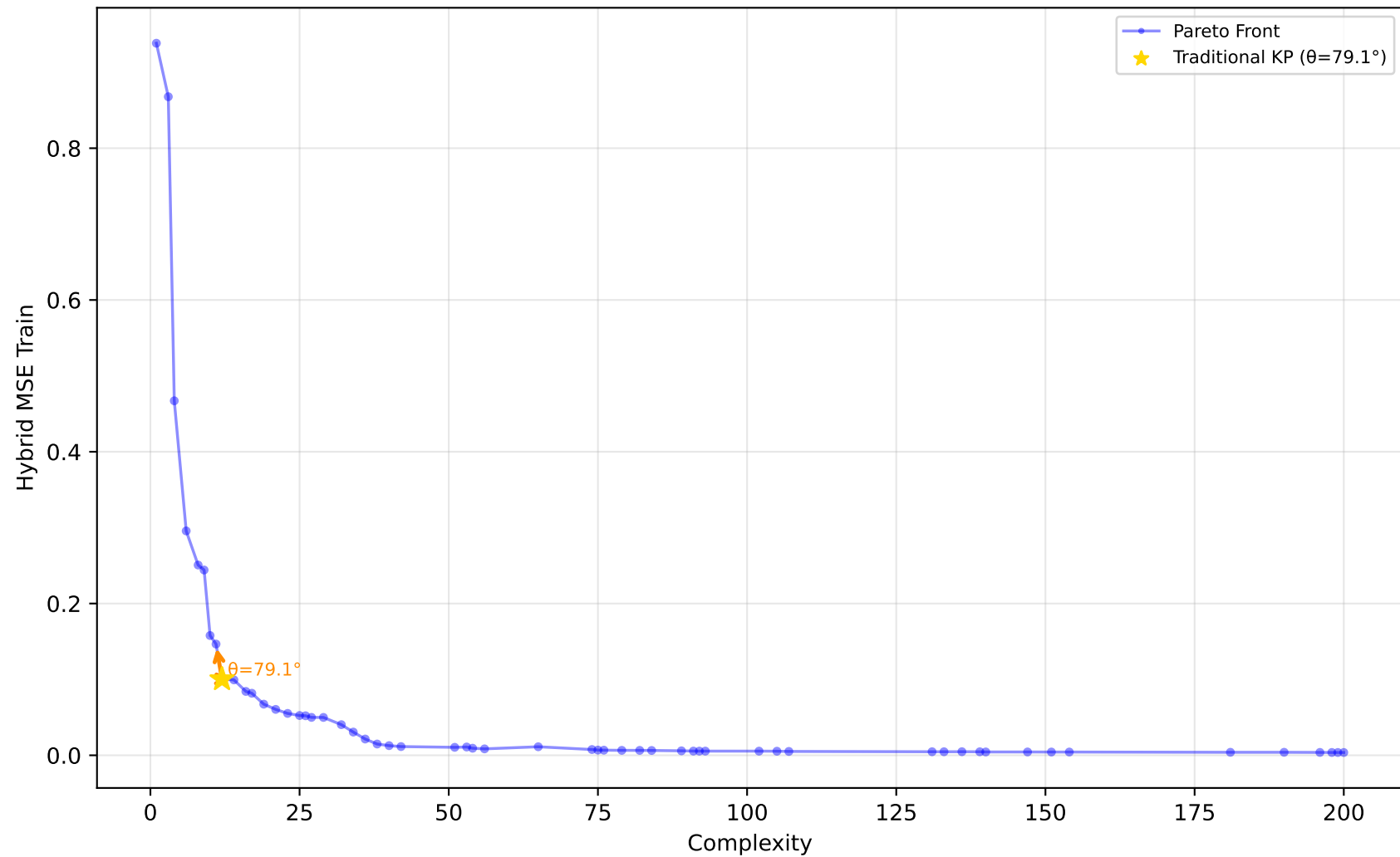
227_cpu_small - Run 22 - SVP - Hybrid MSE Train \lambda_1=0.00, \lambda_2=1.00, \lambda_3=0.00 | Difficulty: 1.00 | Method: hmr
