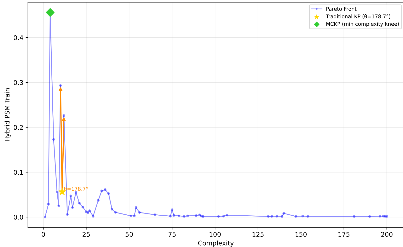
227_cpu_small - Run 22 - SVP - Hybrid PSM Train \lambda_1=0.00, \lambda_2=1.00, \lambda_3=0.00 | Difficulty: 1.00 | Method: hmr
