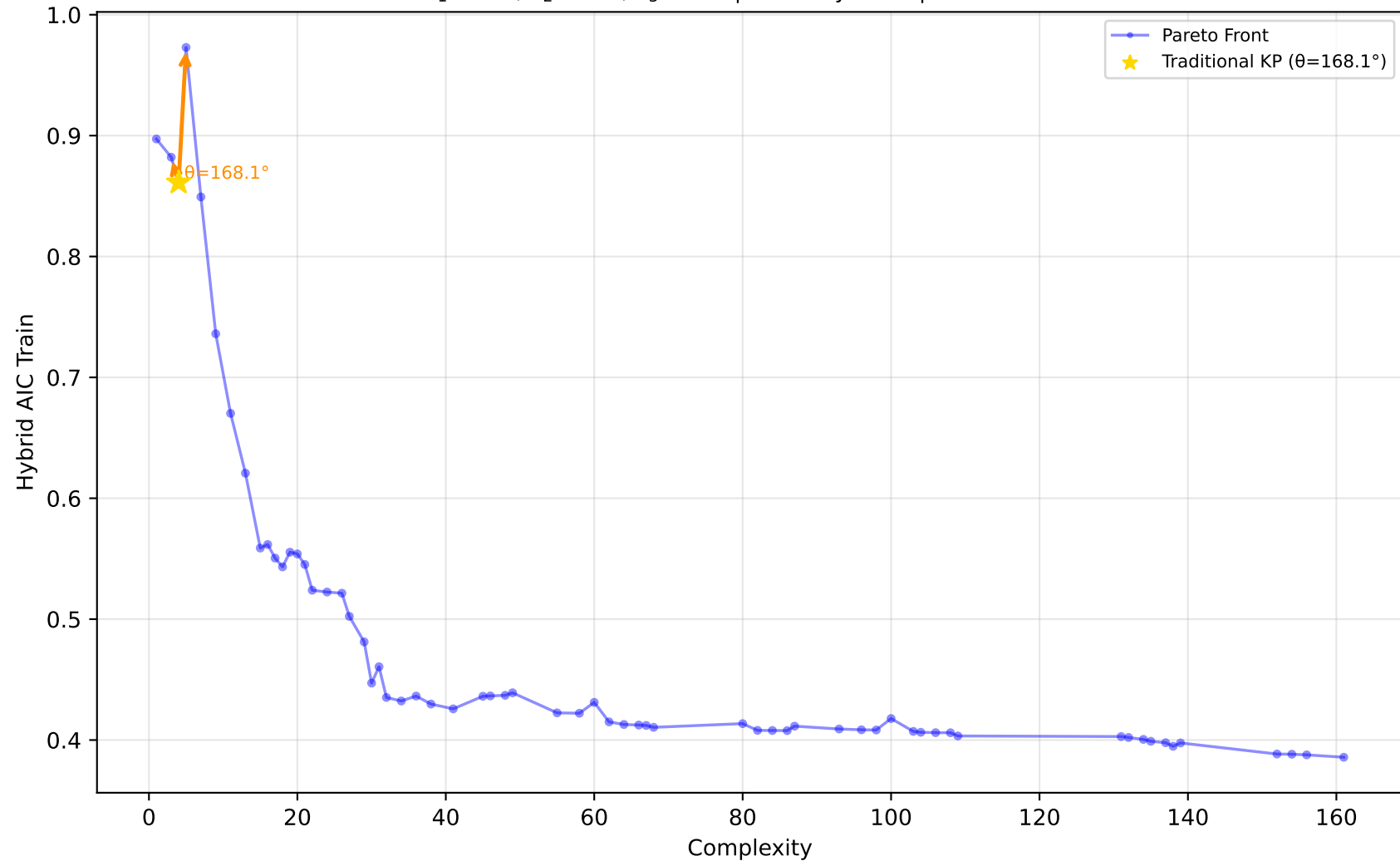
227_cpu_small - Run 23 - MVP - Hybrid AIC Train \lambda_1=0.00, \lambda_2=0.90, \lambda_3=0.10 | Difficulty: 1.00 | Method: hmr
