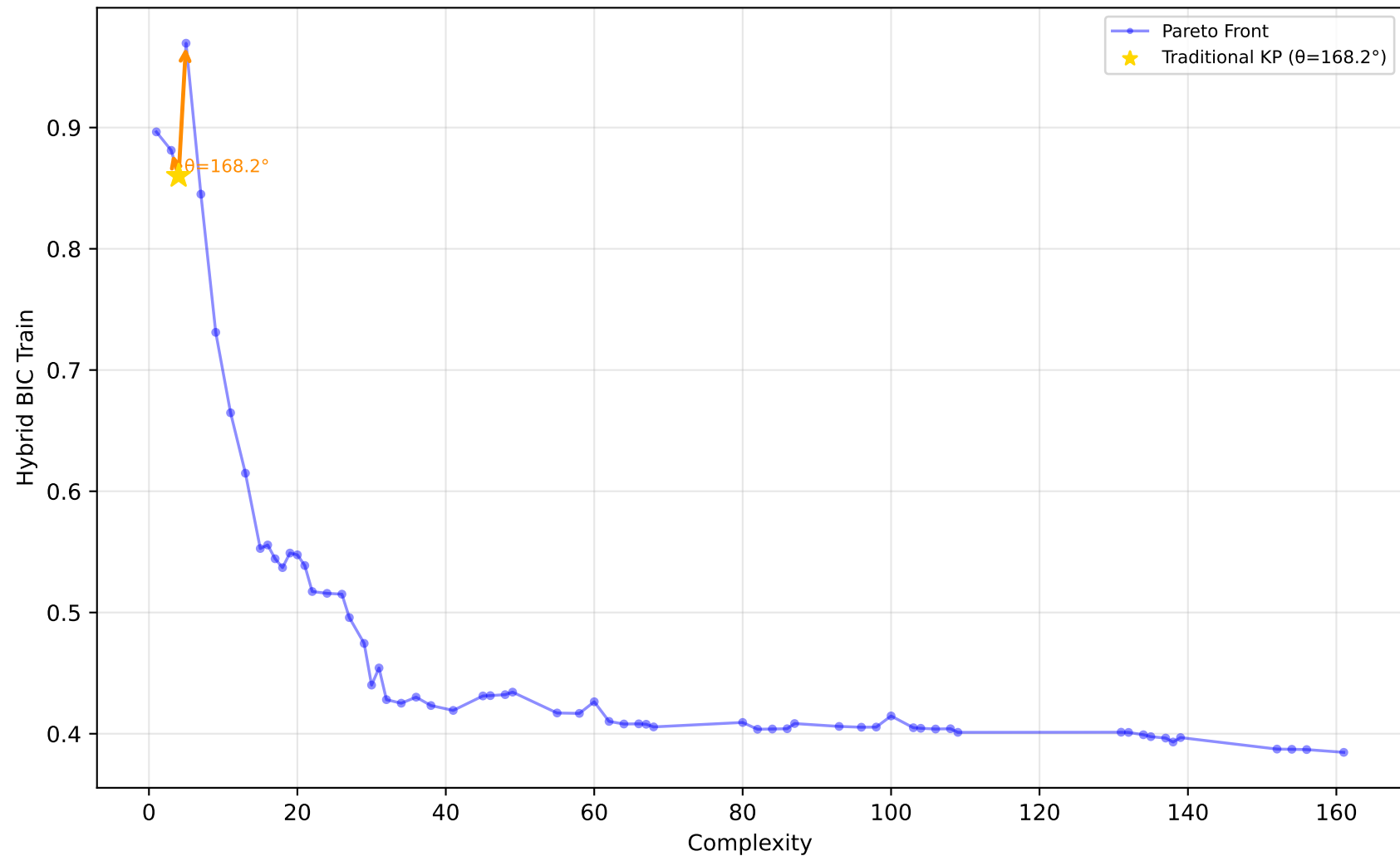
227_cpu_small - Run 23 - MVP - Hybrid BIC Train \lambda_1=0.00, \bar{\lambda}_2=0.90, \lambda_3=0.10 | Difficulty: 1.00 | Method: hmr
