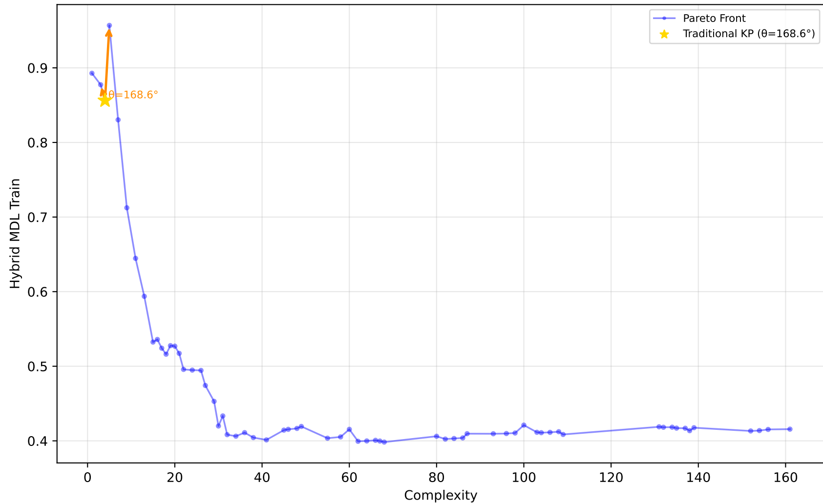
227_cpu_small - Run 23 - MVP - Hybrid MDL Train \lambda_1=0.00, \lambda_2=0.90, \lambda_3=0.10 | Difficulty: 1.00 | Method: hmr
