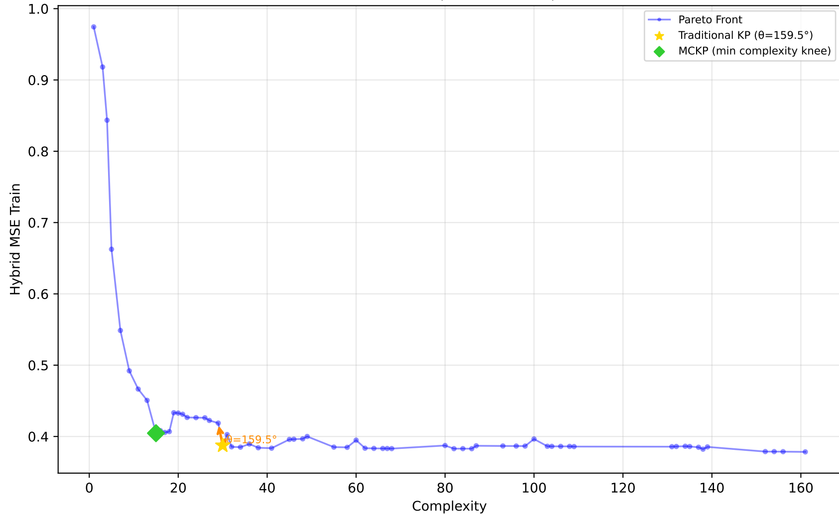
227_cpu_small - Run 23 - MVP - Hybrid MSE Train \lambda_1=0.00, \lambda_2=0.90, \lambda_3=0.10 | Difficulty: 1.00 | Method: hmr
