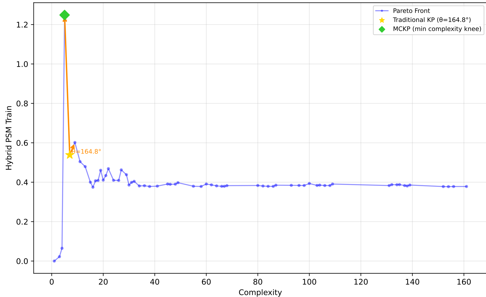
227_cpu_small - Run 23 - MVP - Hybrid PSM Train \lambda_1=0.00, \lambda_2=0.90, \lambda_3=0.10 | Difficulty: 1.00 | Method: hmr
