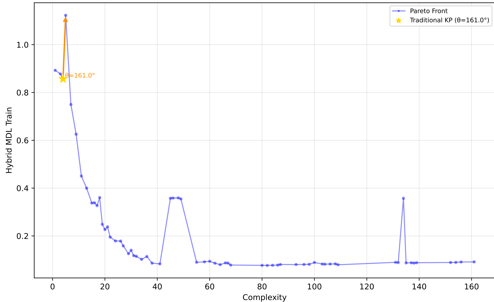
227_cpu_small - Run 23 - SVP - Hybrid MDL Train \lambda_1=0.00, \lambda_2=0.80, \lambda_3=0.30 | Difficulty: 1.00 | Method: hmr
