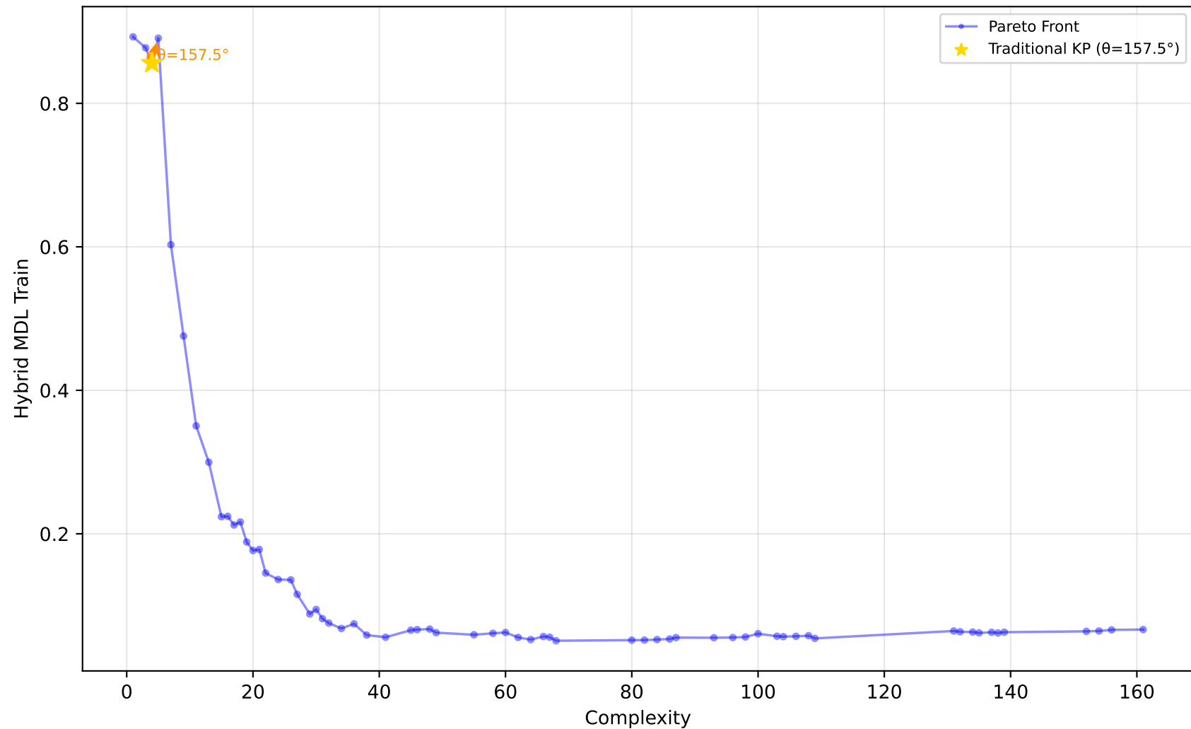
227_cpu_small - Run 23 - SVP - Hybrid MDL Train \lambda_1=0.00, \lambda_2=1.00, \lambda_3=0.00 | Difficulty: 1.00 | Method: hmr
