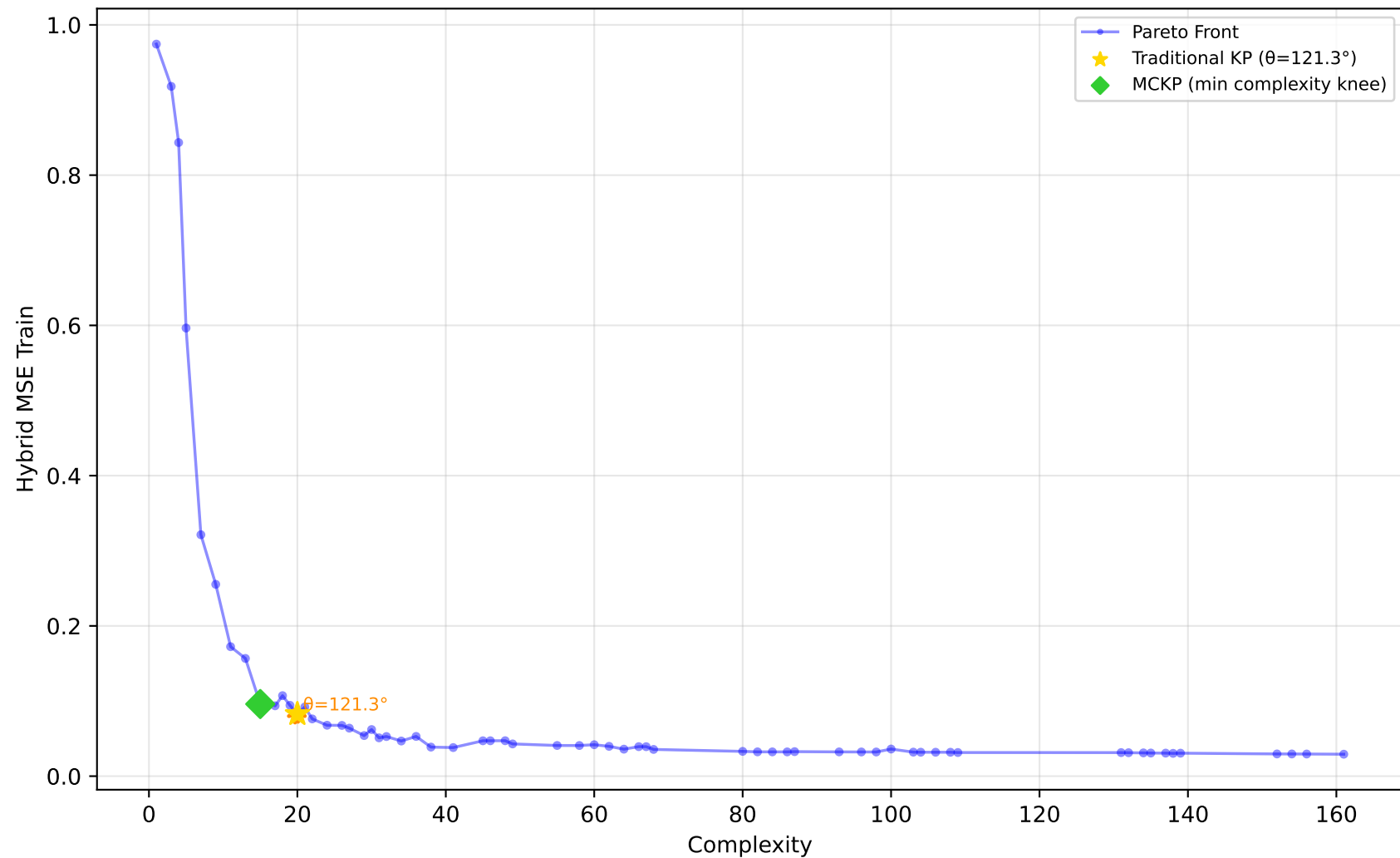
227_cpu_small - Run 23 - SVP - Hybrid MSE Train \lambda_1=0.00, \lambda_2=1.00, \lambda_3=0.00 | Difficulty: 1.00 | Method: hmr
