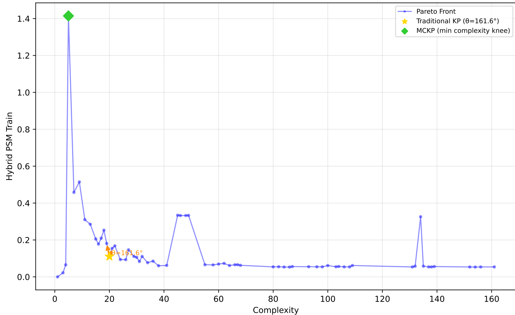
227_cpu_small - Run 23 - SVP - Hybrid PSM Train \lambda_1=0.00, \lambda_2=0.80, \lambda_3=0.30 | Difficulty: 1.00 | Method: hmr
