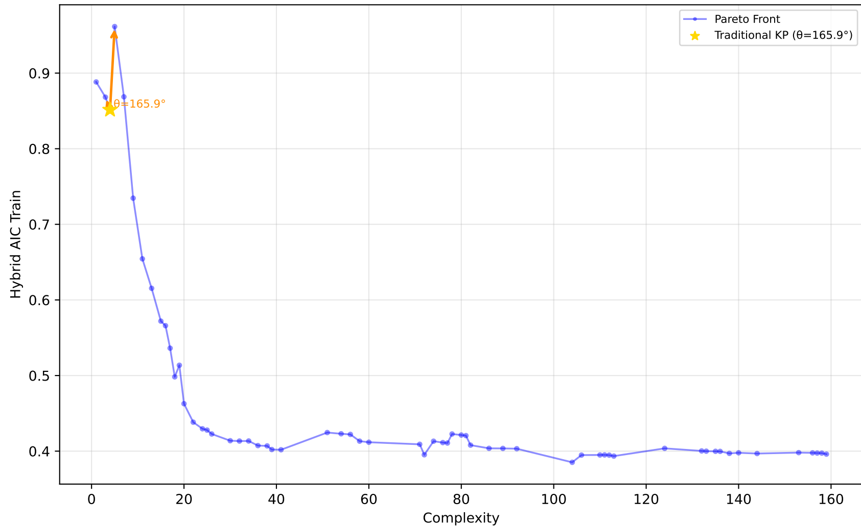
227_cpu_small - Run 24 - MVP - Hybrid AIC Train \lambda_1=0.00, \bar{\lambda}_2=0.90, \lambda_3=0.10 | Difficulty: 1.00 | Method: hmr
