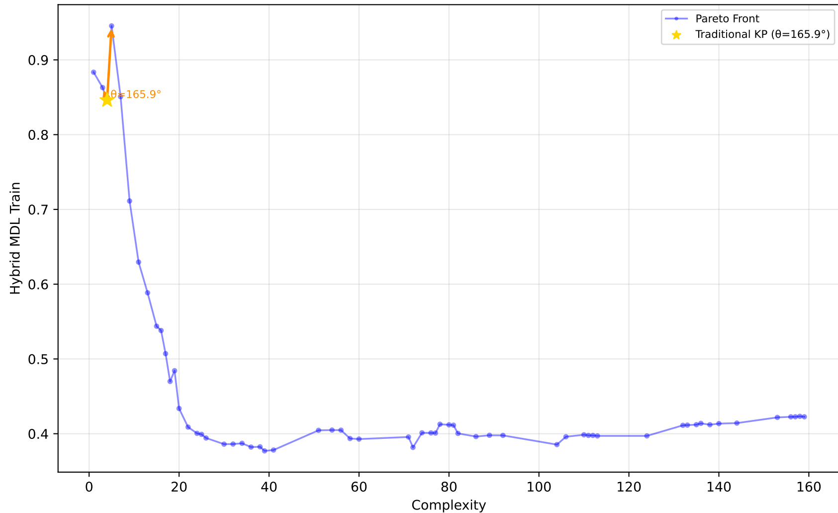
227_cpu_small - Run 24 - MVP - Hybrid MDL Train \lambda_1=0.00, \lambda_2=0.90, \lambda_3=0.10 | Difficulty: 1.00 | Method: hmr
