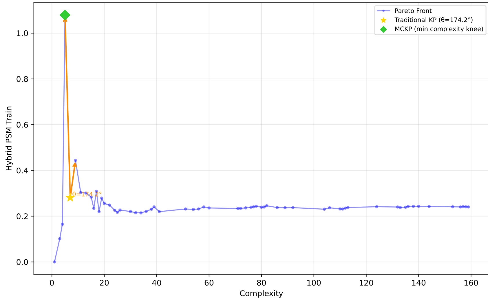
227_cpu_small - Run 24 - MVP - Hybrid PSM Train \lambda_1=0.80, \lambda_2=0.20, \lambda_3=0.00 | Difficulty: 1.00 | Method: hmr
