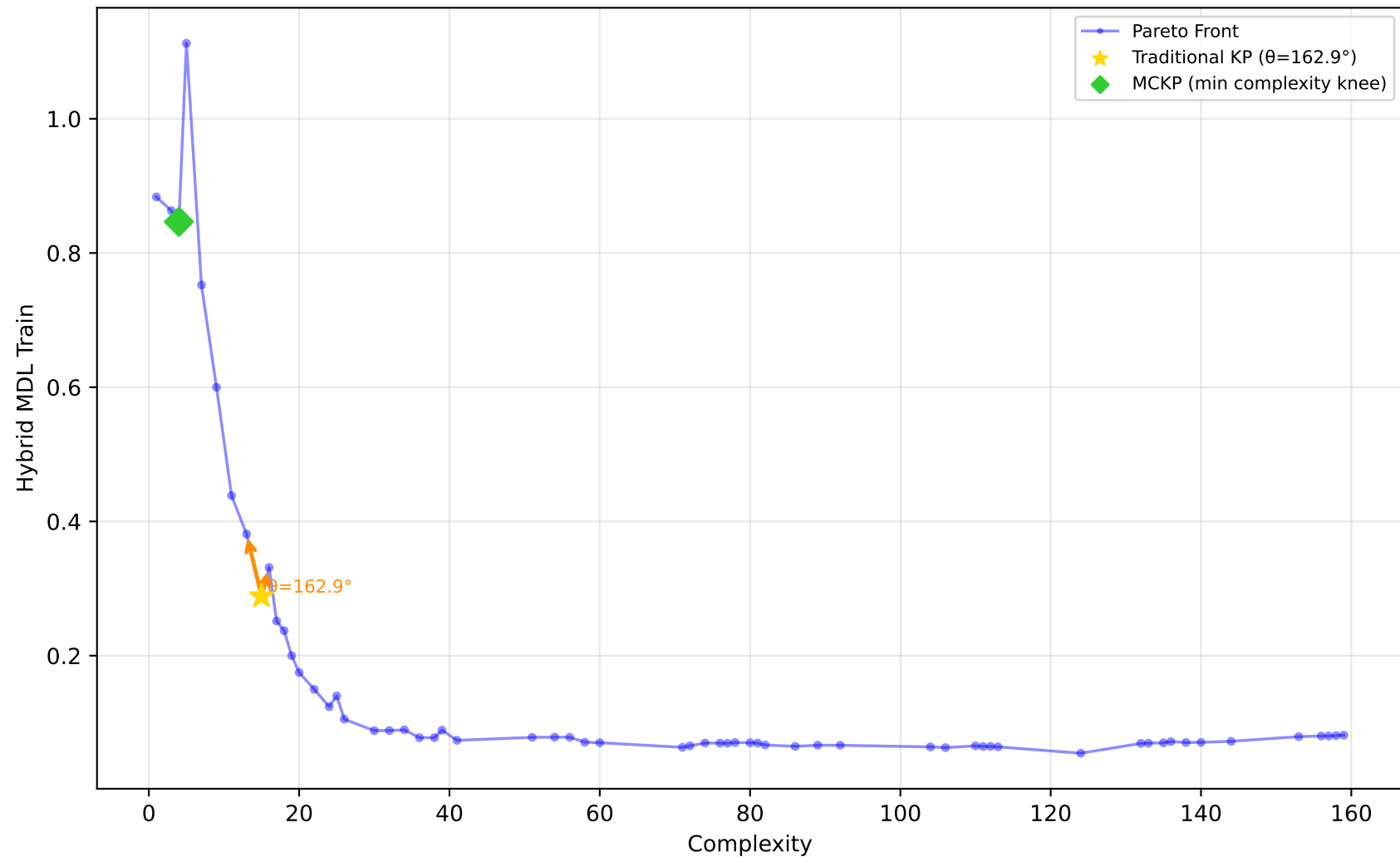
227_cpu_small - Run 24 - SVP - Hybrid MDL Train \lambda_1=0.00, \lambda_2=0.80, \lambda_3=0.30 | Difficulty: 1.00 | Method: hmr
