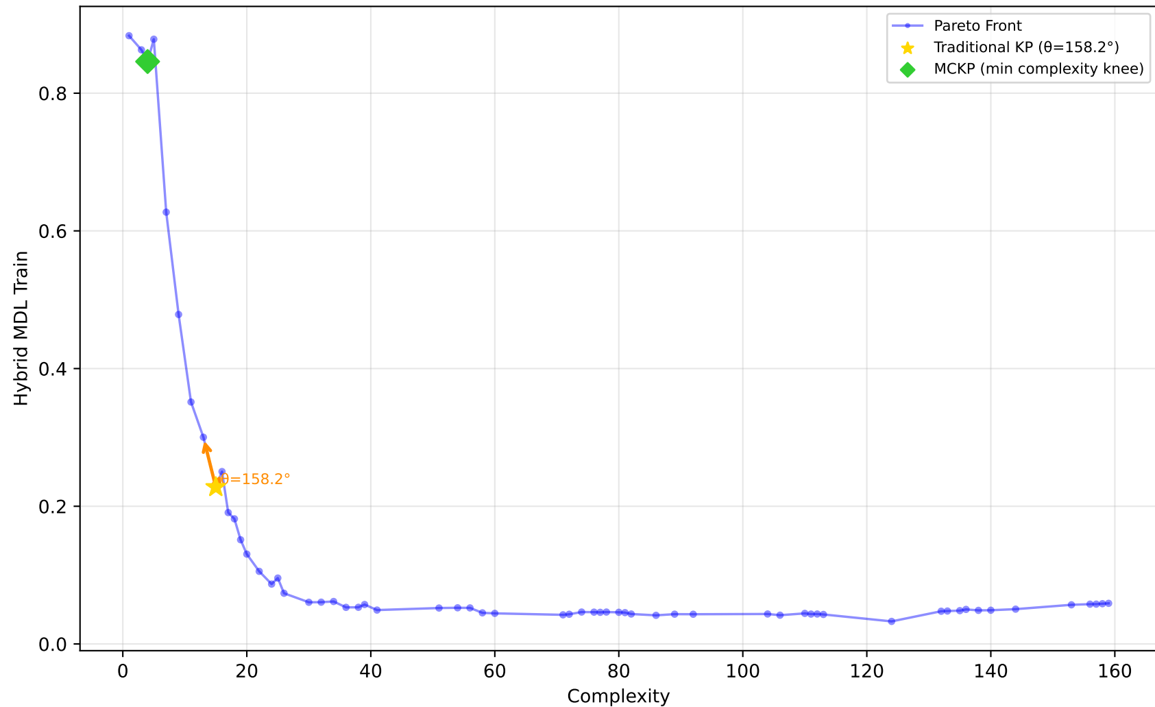
227_cpu_small - Run 24 - SVP - Hybrid MDL Train \lambda_1=0.00, \lambda_2=1.00, \lambda_3=0.00 | Difficulty: 1.00 | Method: hmr
