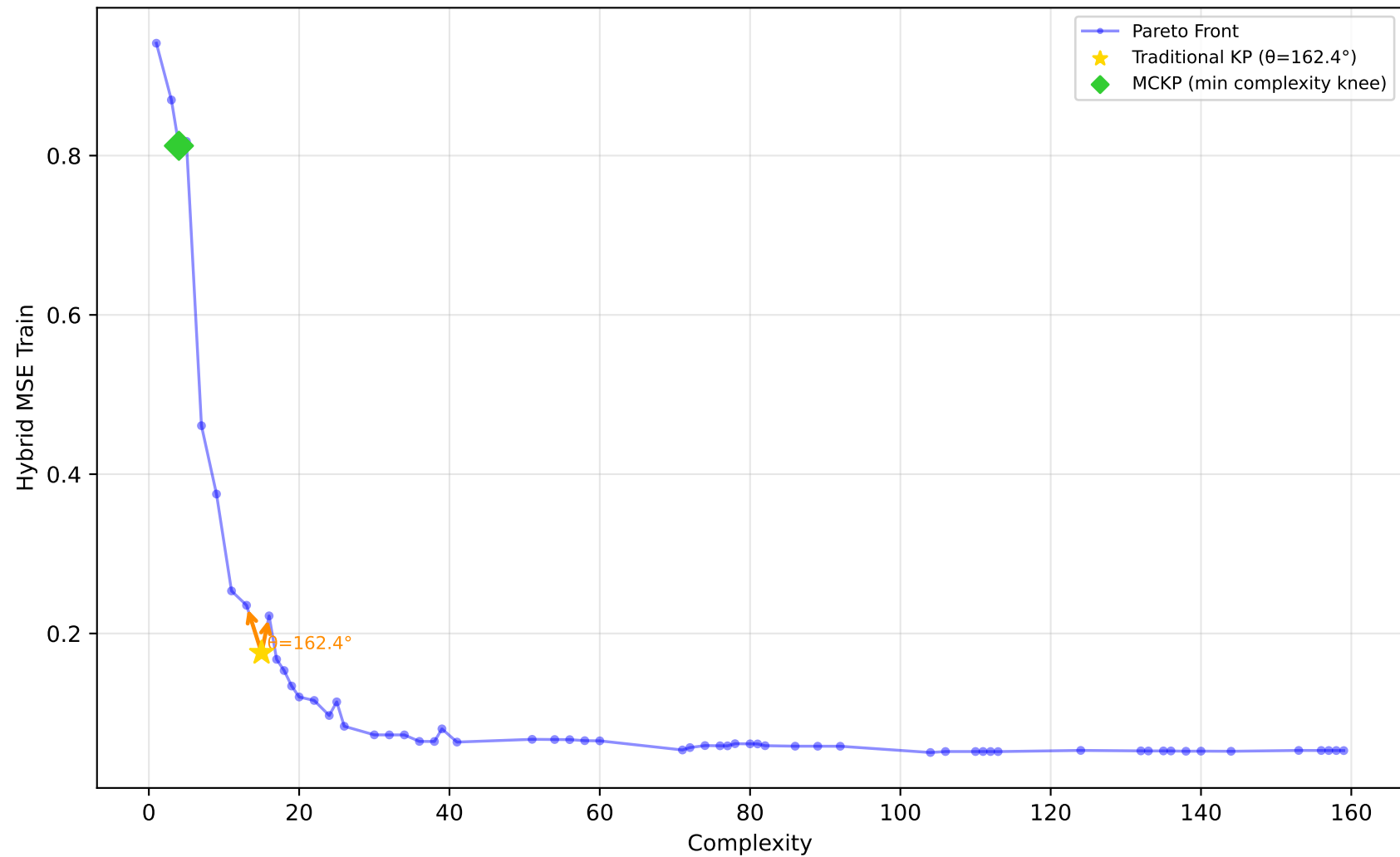
227_cpu_small - Run 24 - SVP - Hybrid MSE Train \lambda_1=0.00, \lambda_2=0.80, \lambda_3=0.30 | Difficulty: 1.00 | Method: hmr
